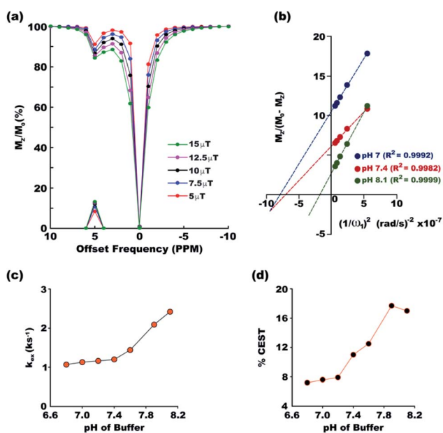
Fig. 3 (a) Overlaid z-spectra of paracetamol at different irradiation powers with 3 s saturation in the physiological condition. The peaks on the x-axis show corresponding MTR_{\text{asym}} . (b) The linear fit for M_z/(M_0 - M_z) plotted against 1/\omega_1^2 for three pH values, 7, 7.4 and 8.1. The goodness of fitting is given by the R^2 values. Plots at other pH values are given in Fig. S33–S39 of ESI.† Exchange rate constant (c) and CEST efficiency (d) at different pH of the medium show gradual increase of both at basic pH.
