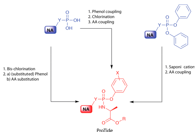
Figure 5. Synthetic strategies for accessing monophosphate ProTides. AA: amino acid. NA: nucleoside analogue. R: any ester. X: any aromatic substitution. Y: O or CH 2 .
