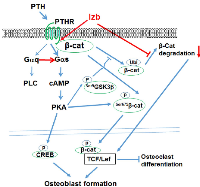
FIGURE 8: Model of Izb regulation of PTHR signaling cascade in bone. Both PTH and Izb are able to induce \beta -catenin ( \beta -Cat)/TCF signaling. Izb stabilizes \beta -Cat by inhibiting its proteasome degradation. \beta -Cat-mediated PTHR signaling switch is blocked by Izb due to its promoting of \beta -Cat translocation, thereby dissociating \beta -Cat from the PTHR. Izb facilitates PTH stimulation of CREB phosphorylation, \beta -Cat (Ser-675) phosphorylation, GSK3 \beta (Ser-9) phosphorylation, and TCF/Lef activity through a cAMP/PKA signaling pathway. Collectively these findings suggest that the combination of PTH and Izb favors the anabolic PTH action in bone.
