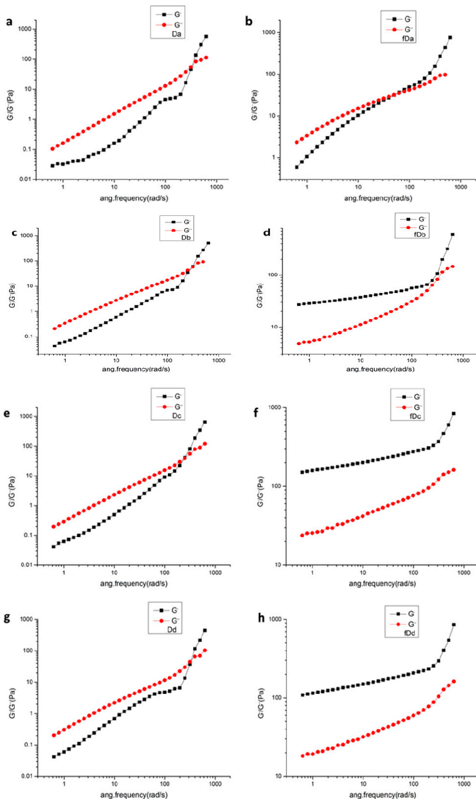
Figure 6. Frequency dependence of G' and G'' of KGM sols with different alkali addition before freezing (a,c,e,g) and after freezing (b,d,f,h) dealt.
