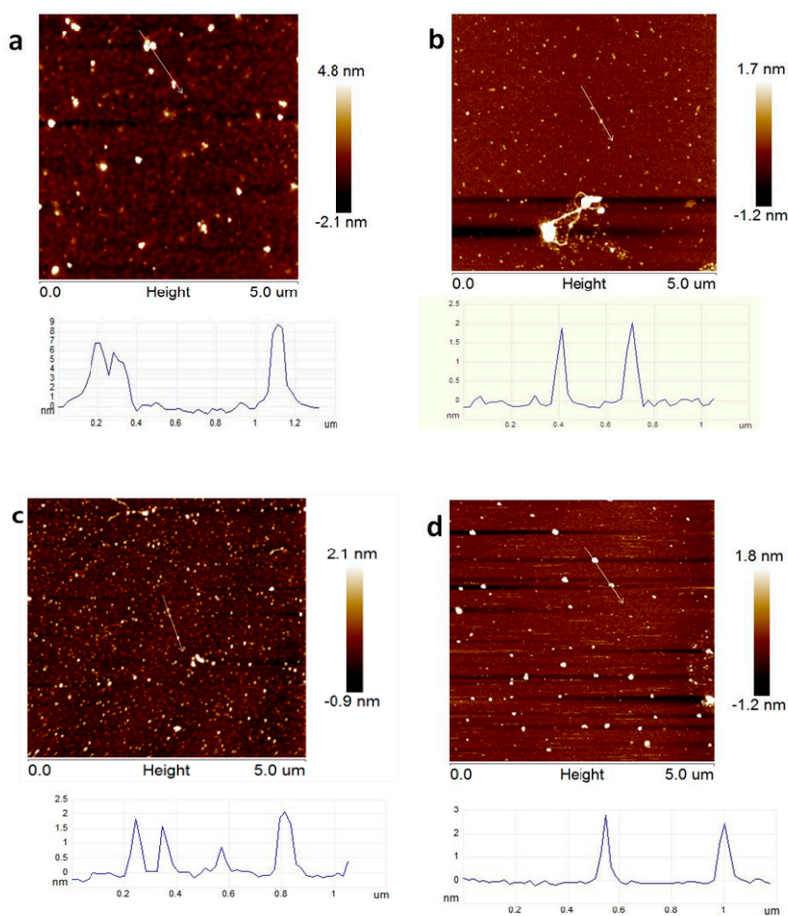
Figure 2. AFM image of KGM treated with different ultrasonic time (image size = 5 \times 5 \mu\text{m} ); (a) non-sonication, (b) 15 min, (c) 30 min, (d) 60 min.
