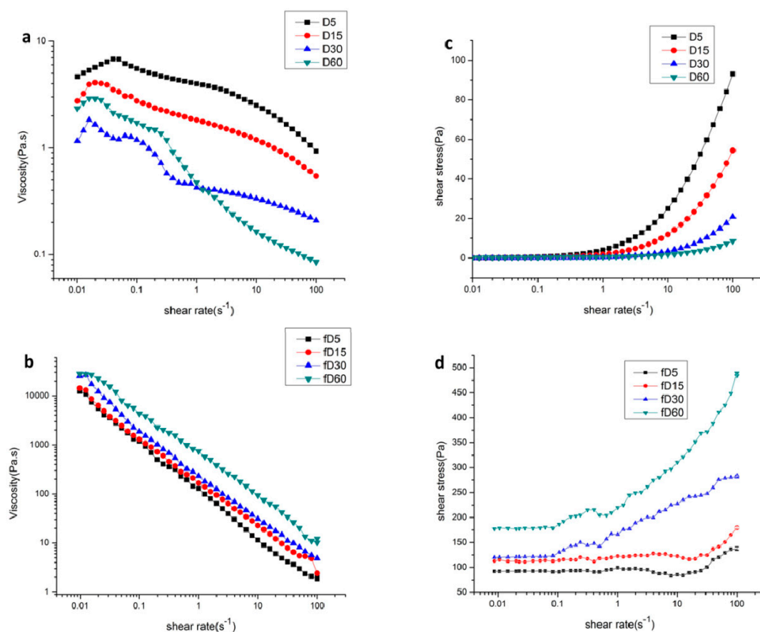
Figure 7. The steady state flow curves of 1% KGM sols with different sonication time before and after freezing dealt.
