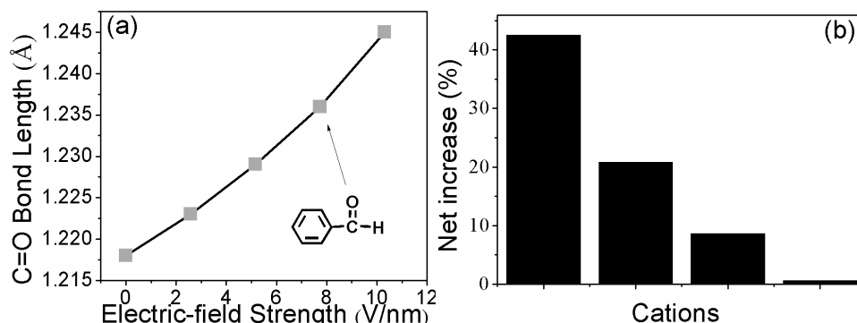
Figure 3 | (a) The relationship between the C=O bond length (Angstrom) of benzaldehyde and the intensity of extra electrostatic fields simulated by the density functional theory (DFT) method. (b) The net increase of the conversion of the condensation reaction between benzaldehyde and 1-pentanol was calculated from Table 1. The net increase means the conversion on Au/MZSM-5 deducts the conversion on its counterpart of MZSM-5 (M = H + , Na + , Ca 2+ , or La 3+ ).
