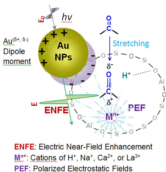
Figure 1 | The acetalization on Au/MZSM-5 ( M = \text{H}^+ , \text{Na}^+ , \text{Ca}^{2+} , or \text{La}^{3+} ) under the irradiation of visible light. ENFE means the electric near-field enhancement of Au-NPs. PEF means the polarized electro-static fields of extra-framework cations in zeolites.
