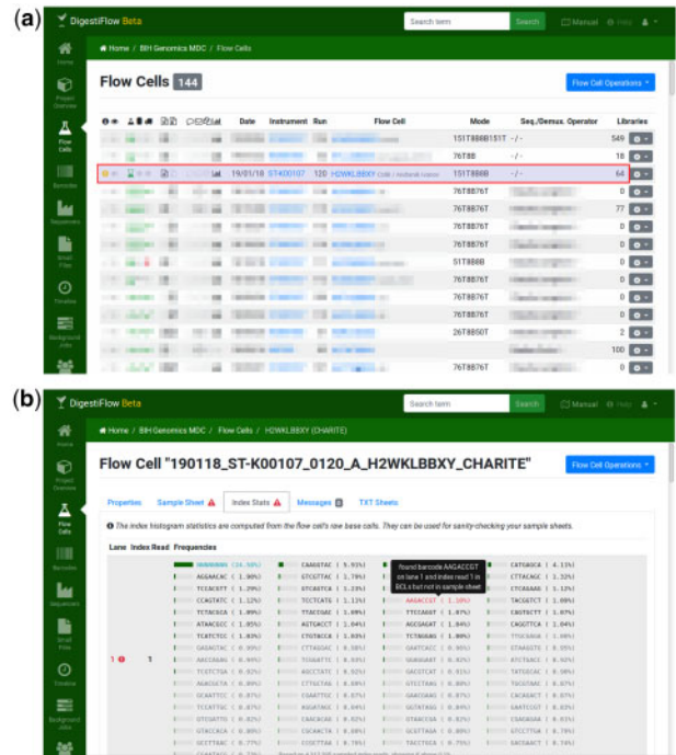
Fig. 2. When adding the sample sheet (not shown), the operator made a small mistake. The adapter P37 is given twice for the same lane in the sample sheet while the adapter sequence ‘AAGACCGT’ occurs in the raw BCLs but not in the sample sheet. This information can then be used for debugging sample sheet information. This is highlighted in the sample sheet (a) and the display of the adapters read from the raw BCL data (b)
