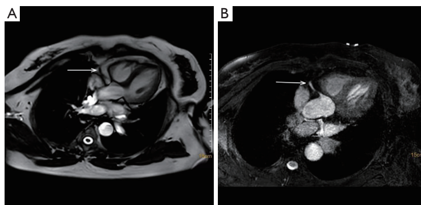
Figure 1 The cine sequence and B-TFE sequence of whole-heart free-breathing NCE-CMRA at 3.0 T from a 70-year-old woman. (A) The axial image of NCE-CMRA scanned by cine sequence. The arrow points to the RCA. (B) The axial image of NCE-CMRA scanned by B-TFE sequence. The arrow points to the RCA. B-TFE, balanced turbo-field-echo; NCE-CMRA, non-contrast-enhanced coronary magnetic resonance angiography; RCA, right coronary artery.
