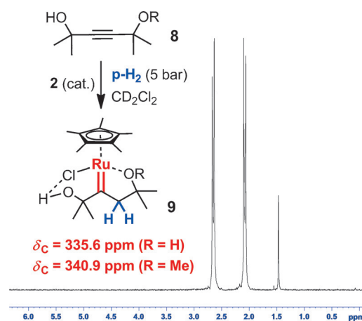
Figure 2. Aliphatic region of the ^1\text{H} -OPSY NMR spectrum showing the gem -coupled protons that must have been delivered pairwise during the hydrogenation of 8a ( R = \text{H} ) with p\text{-H}_2 in the presence of catalytic amounts of complex 2 ; characteristic ^{13}\text{C} NMR data of the resulting carbenes 9a ( R = \text{H} ) and 9b ( R = \text{Me} ).
