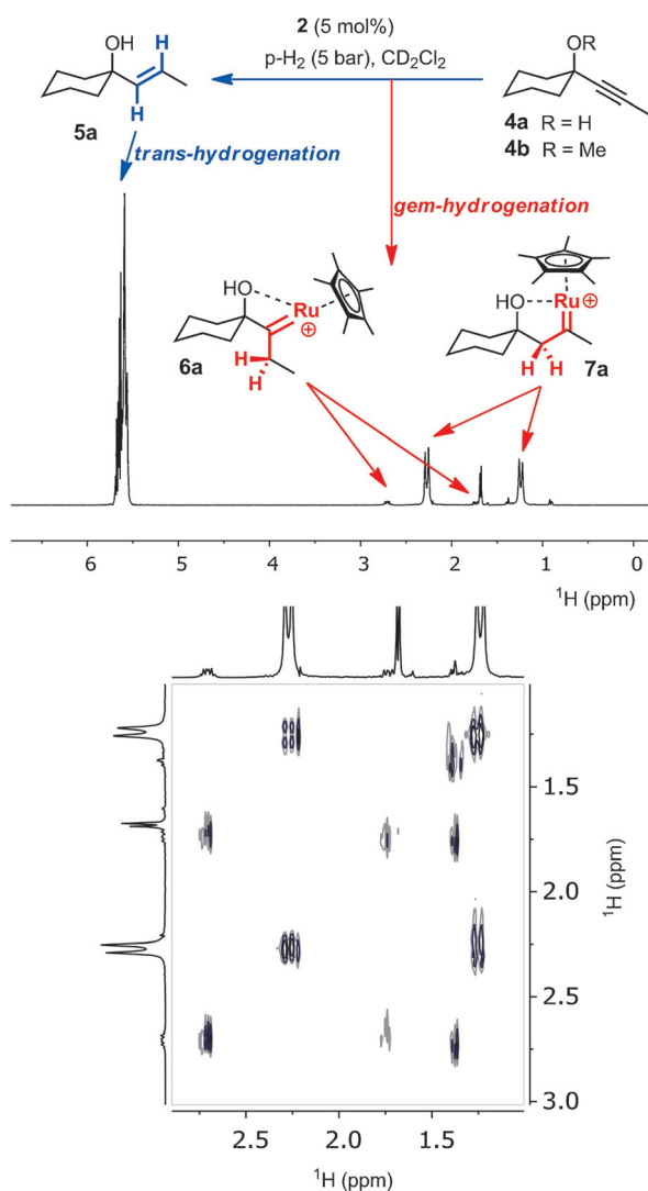
Figure 1. Top: ^1\text{H} -OPSY NMR spectrum taken during the catalytic hydrogenation of 4a ( R = \text{H} ) with p\text{-H}_2 . Bottom: aliphatic region of a ^1\text{H} -OPSY-COSY spectrum, confirming the spin system of the carbene isomers 6a/7a causing the PHIP-enhanced signals. For the assignment of all visible peaks, see the Supporting Information.
