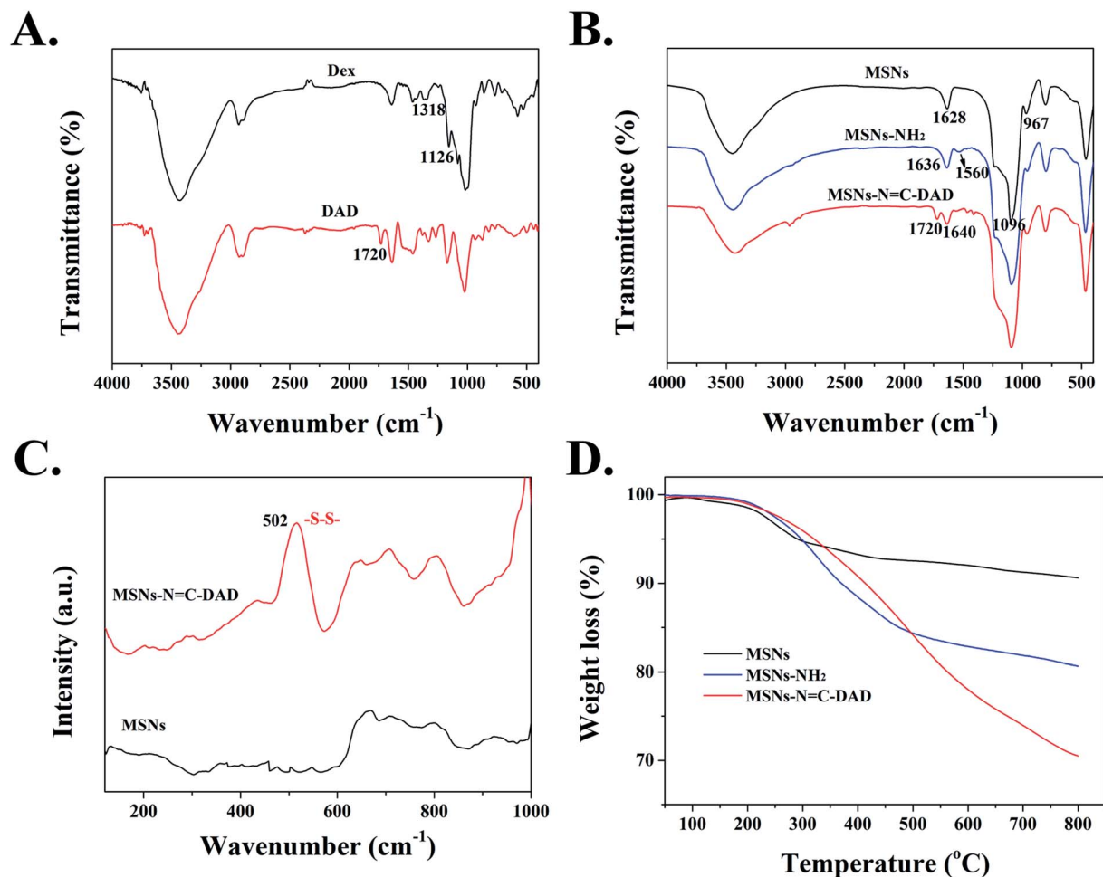
Fig. 2 FTIR spectra of (A) Dex and DAD, (B) MSNs, MSNs-NH 2 and MSNs-N=C-DAD, (C) Raman spectra of MSNs and MSNs-N=C-DAD, and (D) TGA curves of MSNs, MSNs-NH 2 , and MSNs-N=C-DAD.
