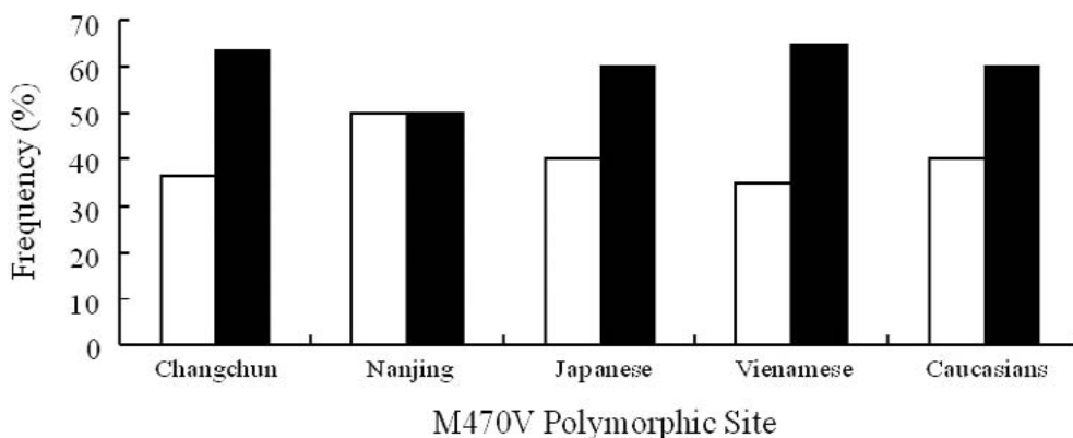
Fig. 2 Frequency of M470V in different populations (The data of Japanese were cited from the paper of Fujiki et al. 9 ) and the data of Vietnamese and Caucasians were cited from the paper of Nam et al. 10 ). White bars are M and black bars are V.
