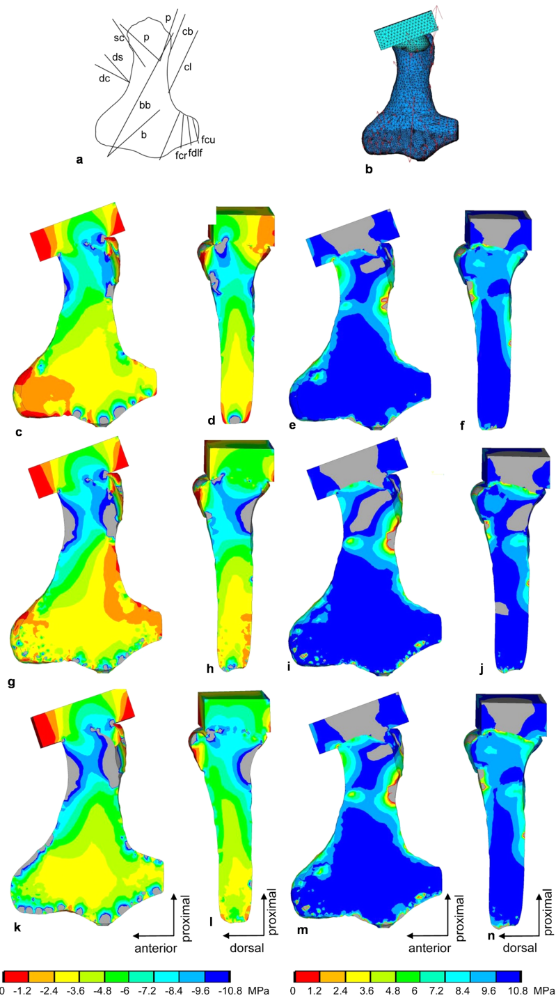
Figure 9 FESA of the humerus of Cryptoclidus eurymerus (IGPB R 324). (A) Outline drawing of the humerus and lines of action of the muscles attaching to it as obtained from the myological analysis. (B) Mesh volumetric FE model with force vectors of attaching muscles (red arrows). (C–F) FESA of load case 1 (downstroke). (G–J) FESA of load case 2 (upstroke). (K–N) FESA superposition of both load cases 1 and 2. The left two columns (C), (D), (G), (H), (K), (L) show the compressive stress distribution, and the right two columns (E), (F), (I), (J), (M), (N) show the tensile stress distribution. The color spectrum indicates the compressive and tensile stress in MPa. Note that the areas of lower compressive stress correspond to the areas of cancellous bone (on the inside of the bone) and the areas of higher compressive
