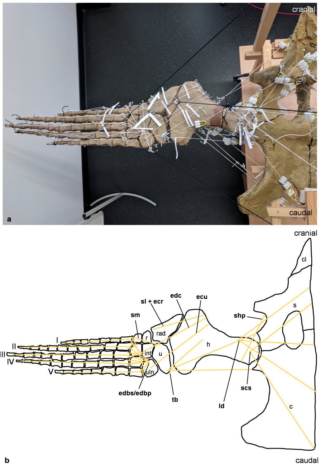
Figure 3 Analog model of the myology of Cryptoclidus eurymerus (mounted skeleton IGPB R 324), shoulder girdle and foreflipper in dorsal view. (A) Mounted bone casts with white chords representing the lines of action of the foreflipper muscles. (B) Tracing of the shoulder girdle and foreflipper with muscle lines of action. Abbreviations of muscles: ecu, musculus extensor carpi ulnaris; edbp/edbs, musculi extensores digitorum breves profundi/musculi extensores digitorum breves superficialis; edc,
