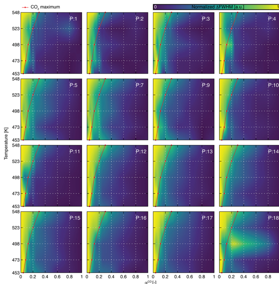
Figure 5. Plasmonic nanospectroscopy of single Pt catalyst nanoparticles. Normalized \Delta\text{FWHM} (details in methods) for 16 individual particles during an \alpha^{\text{CO}} down sweep from 1 to 0 in the temperature interval 453–548 K. The plots are interpolated from measurements performed at five temperatures indicated by the ticks on the y-axis. The red line corresponds to the \alpha^{\text{CO}} -value at which the maximum \text{CO}_2 production is measured by the QMS for each temperature. The color code denotes the normalized amplitude of the \Delta\text{FWHM} response and blue corresponds to a predominantly CO-covered catalyst surface, whereas yellow denotes the O-covered state of the catalyst particle. Particle numbers shown on the upper right of each panel indicate the relative particle position along the model pore, where particle P1 is located most upstream, i.e., toward the inlet (see also Figure 6a).
