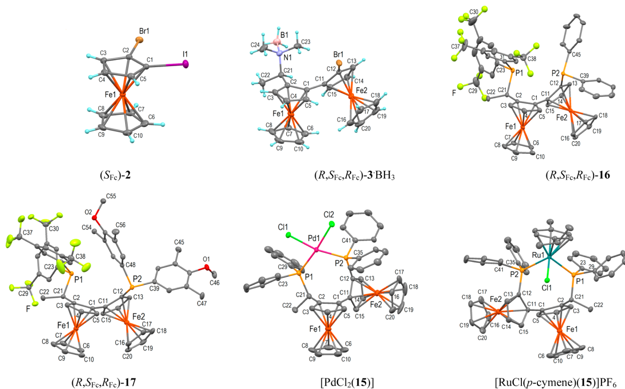
Figure 1. Molecular structures of (S_{Fc}) -2, (R,S_{Fc},R_{Fc}) -3-BH 3 , (R,S_{Fc},R_{Fc}) -16, (R,S_{Fc},R_{Fc}) -17, [PdCl 2 (15)] (molecule 1), and [RuCl( p -cymene)(15)]PF 6 showing 50% displacement ellipsoids. Hydrogen atoms and PF 6 − are omitted for clarity.
