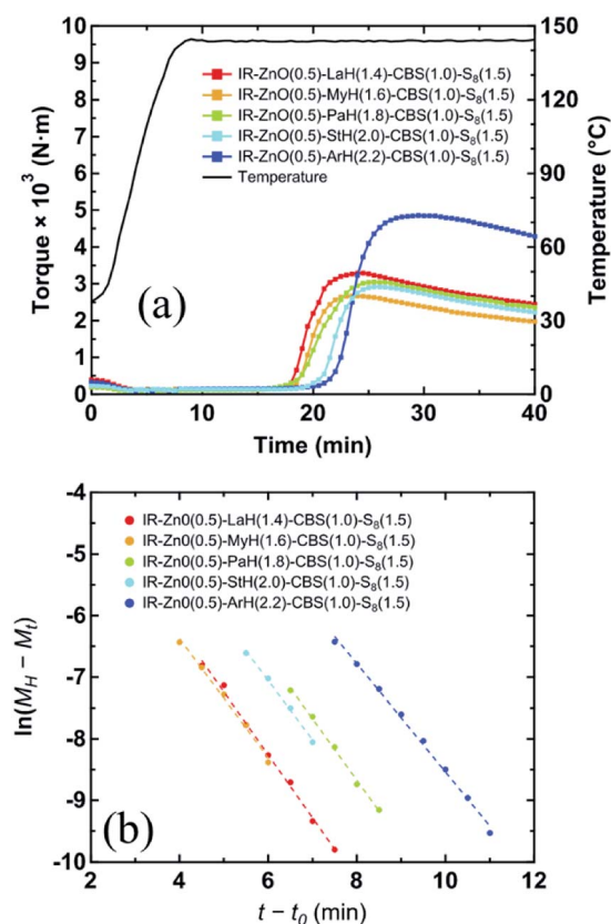
Fig. 9 (a) Cure curves of the samples in the vulcanized system. (b) Variation of \ln(M_{\text{H}} - M_t) plotted against (t - t_0) of the samples.
