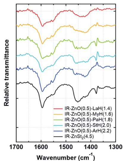
Fig. 3 Differential FT-IR spectra of the samples subtracted using a spectrum of raw isoprene rubber at 144 °C in the range of 1700–1300 cm -1 .
