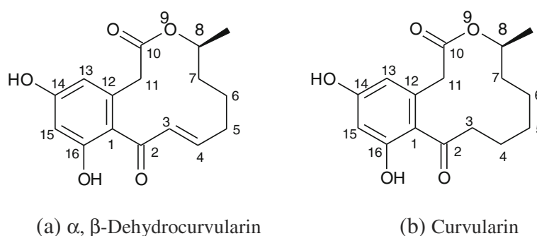
Figure 1 Structures for (a) \alpha , \beta -dehydrocurvularin and (b) curvularin produced by Chrysosporium lobatum strain BK-3.
