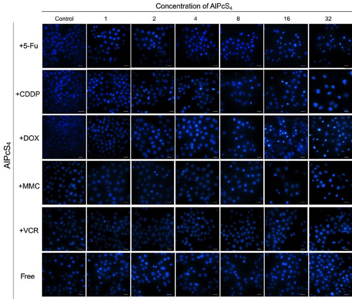
Figure 5. Apoptosis induced by AIPcS 4 +5-FU, AIPcS 4 +CDDP, AIPcS 4 +DOX, AIPcS 4 +MMC, AIPcS 4 +VCR and free-AIPcS 4 in SGC-7901 cells after being irradiated for 24 h. The cells were then treated with 1-32 \mu\text{m}/\text{ml} free-AIPcS 4 or AIPcS 4 +5-FU (20 \mu\text{m} ), AIPcS 4 +CDDP (5 \mu\text{m} ), AIPcS 4 +DOX (0.4 \mu\text{m}/\text{ml} ), AIPcS 4 +MMC (0.5 \mu\text{m}/\text{ml} ) or AIPcS 4 +VCR (0.1 \mu\text{m}/\text{ml} ) for 6 h. The cells were then irradiated with 635-nm laser irradiation at 100 \text{mW}/\text{cm}^2 illumination dosage for 5 min, incubated for 24 h, stained with Hoechst 33342 probe, and then imaged using a fluorescence microscope. All the Hoechst staining images were acquired at an x400 magnification. The scale bar represented 20 \mu\text{m} . AIPcS 4 , Al(III) phthalocyanine chloride tetrasulfonic acid; 5-FU, 5-fluorouracil; DOX, doxorubicin; CDDP, cisplatin; MMC, mitomycin C; VCR, vincristine.
