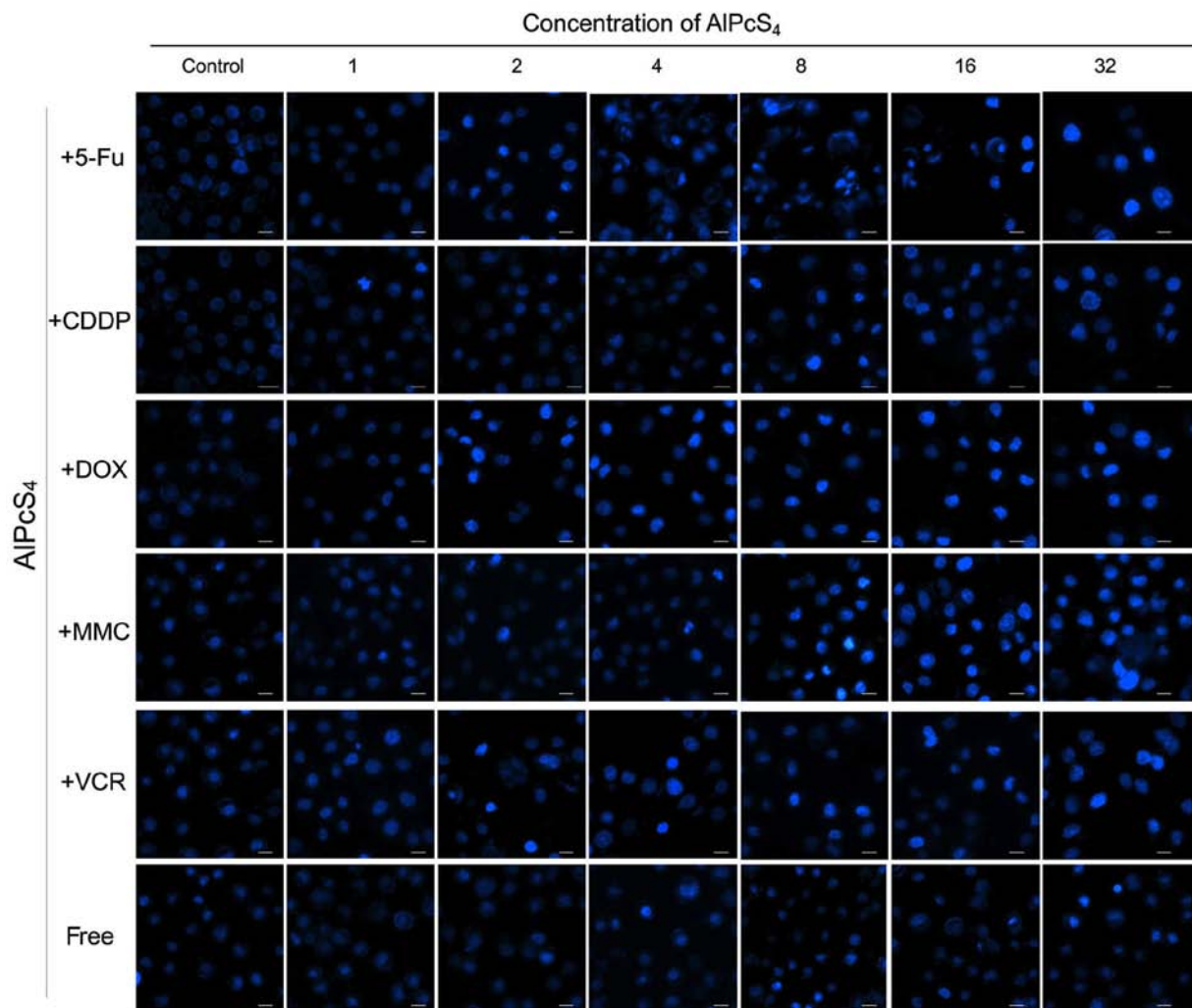
Figure 4. Apoptosis induced by AIPcS 4 +5-FU, AIPcS 4 +CDDP, AIPcS 4 +DOX, AIPcS 4 +MMC, AIPcS 4 +VCR, and free-AIPcS 4 in SGC-7901 cells after being irradiated for 12 h. The cells were treated with 1-32 \mu\text{m}/\text{ml} free-AIPcS 4 or AIPcS 4 +5-FU (20 \mu\text{m} ), AIPcS 4 +CDDP (5 \mu\text{m} ), AIPcS 4 +DOX (0.4 \mu\text{m}/\text{ml} ), AIPcS 4 +MMC (0.5 \mu\text{m}/\text{ml} ) or AIPcS 4 +VCR (0.1 \mu\text{m}/\text{ml} ) for 6 h. The cells were then irradiated with 635-nm laser irradiation at 100 \text{mw}/\text{cm}^2 illumination dosage for 5 min, incubated for 12 h, stained with Hoechst 33342 probe, and then imaged using a fluorescence microscope. All the Hoechst staining images were acquired at an x400 magnification. The scale bar represented 20 \mu\text{m} . AIPcS 4 , Al(III) phthalocyanine chloride tetrasulfonic acid; 5-FU, 5-fluorouracil; DOX, doxorubicin; CDDP, cisplatin; MMC, mitomycin C; VCR, vincristine.
