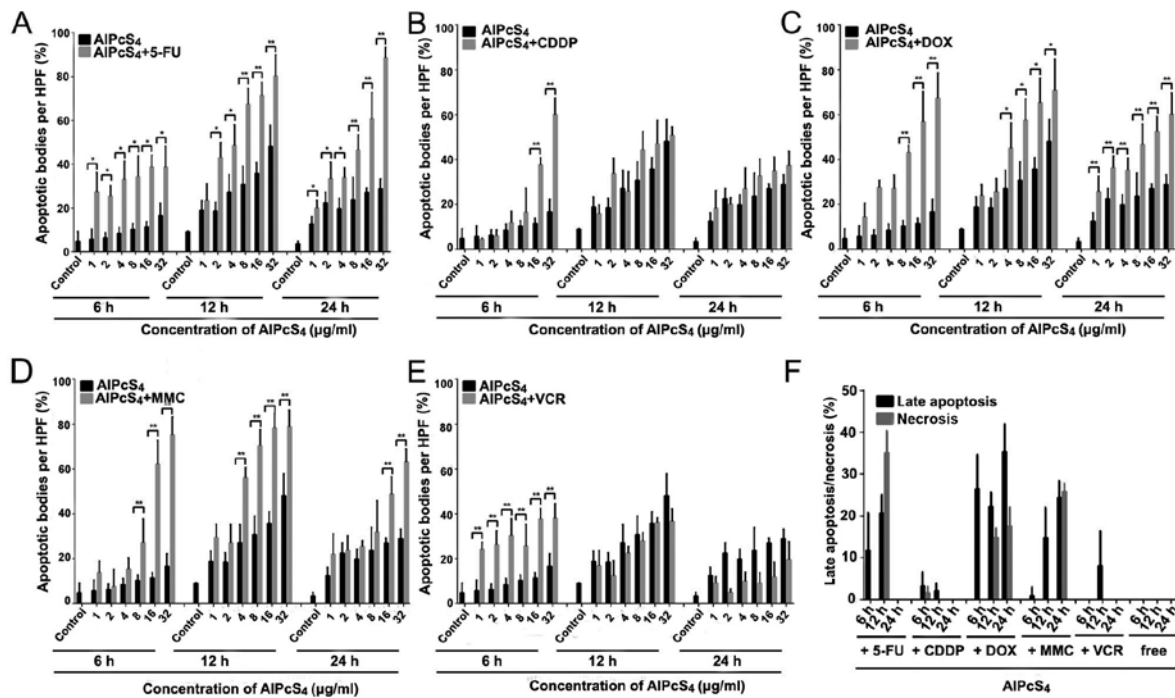
Figure 7. Statistical analysis of apoptosis and necrosis induced by AIPcS 4 +5-FU, AIPcS 4 +CDDP, AIPcS 4 +DOX, AIPcS 4 +MMC, AIPcS 4 +VCR and free-AIPcS 4 in SGC-7901 cells after being irradiated for 6, 12 and 24 h. (A-E) The histograms represent the percentage of cells with apoptotic and necrotic characteristics among 200 cells at a high-power field. The data represent the average of three experiments. The bar is the SD. *P<0.05 and **P<0.01 represented a statistically significant difference in the number of apoptotic bodies between the combination of AIPcS 4 with a chemical agent and free-AIPcS 4 . AIPcS 4 , Al(III) phthalocyanine chloride tetrasulfonic acid; 5-FU, 5-fluorouracil; DOX, doxorubicin; CDDP, cisplatin; MMC, mitomycin C; VCR, vincristine.
