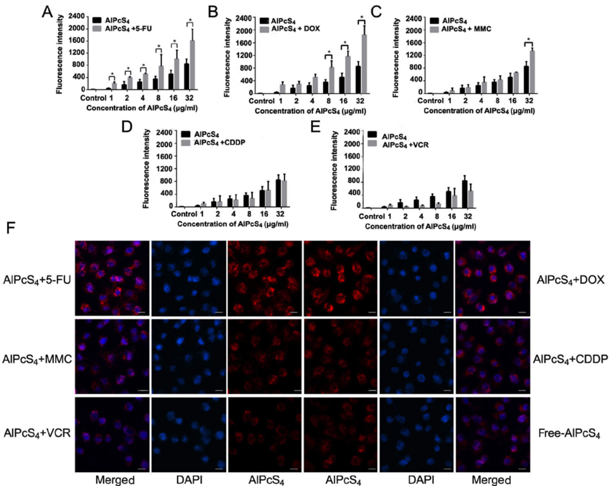
Figure 8. Fluorescence intensity analysis and fluorescence imaging of AIPcS 4 in SGC-7901 cells after treatment with AIPcS 4 + 5-FU, AIPcS 4 + DOX, AIPcS 4 + MMC, AIPcS 4 + CDDP, AIPcS 4 + VCR and free-AIPcS 4 . (A-E) Fluorescent intensity analysis of AIPcS 4 in SGC-7901 cells after treatment with 1-32 µm/ml free-AIPcS 4 , AIPcS 4 + 5-FU (20 µm), AIPcS 4 + DOX (0.4 µm), AIPcS 4 + MMC (0.5 µm/ml), AIPcS 4 + CDDP (5 µm) or AIPcS 4 + VCR (0.1 µm/ml) for 6 h and measured by using a fluorescence spectrophotometer. The data represents the average of three experiments and the bar is the SD. *P<0.05 and **P<0.01 represented a statistically significant difference in the fluorescence intensity of AIPcS 4 in cells between the combination therapy of AIPcS 4 with a chemical agent and single therapy of free-AIPcS 4 . (F) The fluorescent images of AIPcS 4 in SGC-7901 cells after treatment with 32 µm/ml free-AIPcS 4 , AIPcS 4 + 5-FU (20 µm), AIPcS 4 + DOX (0.4 µm/ml), AIPcS 4 + MMC (0.5 µm/ml), AIPcS 4 + CDDP (5 µm) or AIPcS 4 + VCR (0.1 µm/ml) for 6 h and measured using a fluorescence microscope. All the images were acquired at an x400 magnification. The scale bar represented 20 µm. AIPcS 4 , Al(III) phthalocyanine chloride tetrasulfonic acid; 5-FU, 5-fluorouracil; DOX, doxorubicin; CDDP, cisplatin; MMC, mitomycin C; VCR, vincristine.
