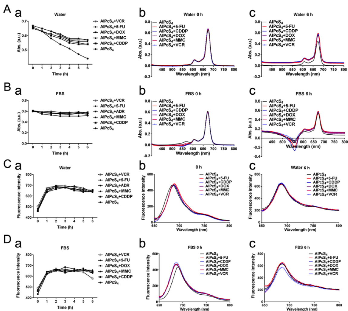
Figure 1. UV-vis absorption spectra and fluorescence intensity of AIPcS 4 mixture with 5-FU (20 \mu\text{M} ), CDDP (5 \mu\text{M} ), DOX (0.4 \mu\text{M} /ml), MMC (0.5 \mu\text{M} /ml), and VCR (0.1 \mu\text{M} /ml) or free-AIPcS 4 at 8 \mu\text{M} /ml. (A-a and B-a) Maximum OD values near 675 nm absorption spectra of corresponding agents in deionized water and RPMI-1640 culture medium that contained FBS at 1-6 h. (A-b and B-b) UV-vis absorption spectra of corresponding agents in deionized water and RPMI-1640 culture medium that contained FBS at 0 h. (A-c and B-c) UV-Vis absorption spectra of corresponding agents in deionized water and RPMI-1640 culture medium that contained FBS at 6 h. (C-a and D-a) Maximum fluorescence intensity near 687 nm fluorescence spectra of corresponding agents in deionized water and RPMI-1640 culture medium that contained FBS at 1-6 h. (C-b and D-b) Fluorescence spectra of corresponding agents in deionized water and RPMI-1640 culture medium that contained FBS at 0 h. (C-c and D-c) Fluorescence spectra of corresponding agents in deionized water and RPMI-1640 culture medium that contained FBS at 6 h. AIPcS 4 , Al(III) phthalocyanine chloride tetrasulfonic acid; 5-FU, 5-fluorouracil; DOX, doxorubicin; CDDP, cisplatin; MMC, mitomycin C; VCR, vincristine; ROS.
