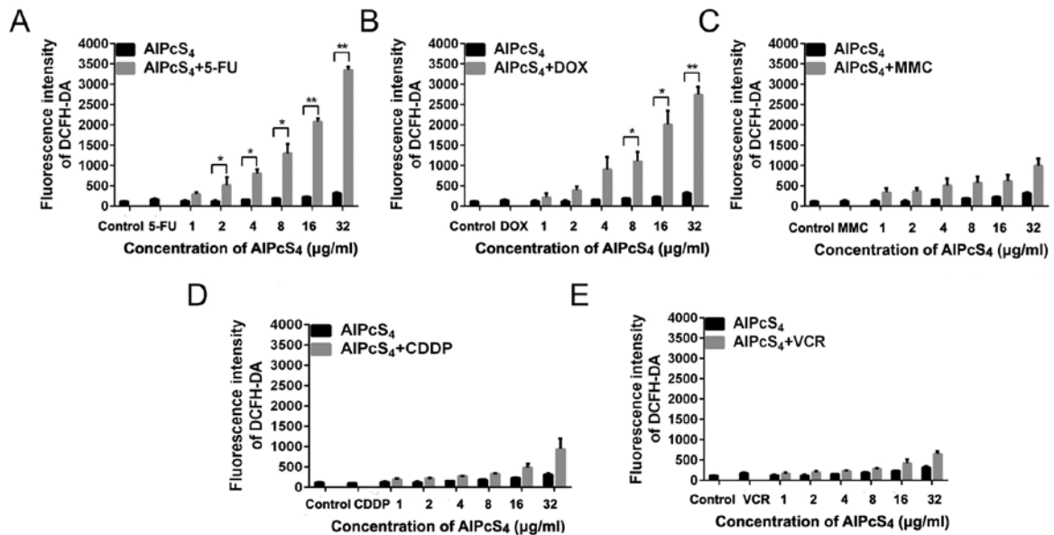
Figure 10. ROS production in SGC-7901 cells treated with AIPcS 4 +5-FU, AIPcS 4 +CDDP, AIPcS 4 +DOX, AIPcS 4 +MMC, AIPcS 4 +VCR and free-AIPcS 4 . (A-E) Fluorescence intensities of DCFH-DA probes were measured to analyze ROS in SGC-7901 cells after treatment with 1-32 µm/ml free-AIPcS 4 . (A) AIPcS 4 +5-FU (20 µm/ml), (B) AIPcS 4 +DOX (0.4 µm/ml), (C) AIPcS 4 +MMC (0.5 µm/ml), (D) AIPcS 4 +CDDP (5 µm) or (E) AIPcS 4 +VCR (0.1 µm/ml) and irradiation with 635-nm laser light for 5 min. Data represent the average of three experiments and the bar is the SD. *P<0.05 and **P<0.01 represent a statistically significant difference in the fluorescence intensity of DCFH-DA in cells between the combination therapy of AIPcS 4 with a chemical agent and single therapy of free-AIPcS 4 . AIPcS 4 , Al(III) phthalocyanine chloride tetrasulfonic acid; 5-FU, 5-fluorouracil; DOX, doxorubicin; CDDP, cisplatin; MMC, mitomycin C; VCR, vincristine; ROS, reactive oxygen species.
