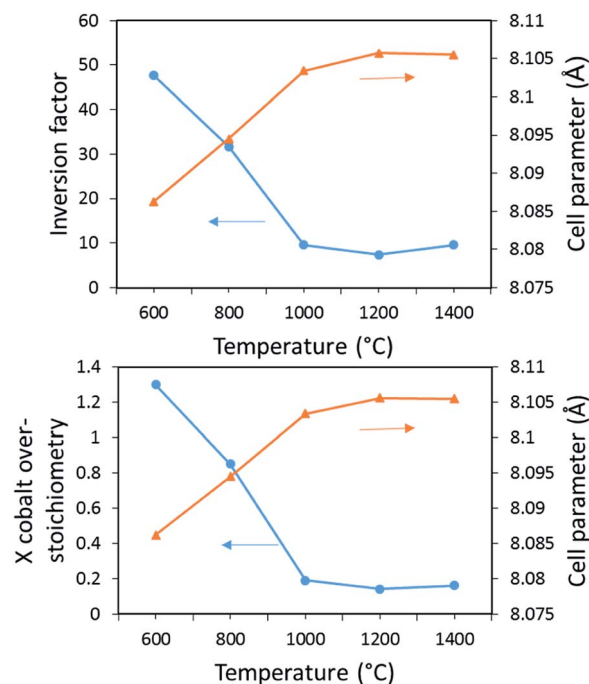
Fig. 3 (Top figure) Unit-cell parameter ( \blacktriangle ) and the \zeta inversion factor ( \bullet ) in \text{Co}_{1-\zeta}\text{Al}_2[\text{Co}_\zeta\text{Al}_{2-\zeta}]\text{O}_4 compounds issued from the 1 st refinement process. (Bottom figure) Unit-cell parameter ( \blacktriangle ) and x cobalt over-stoichiometry ( \bullet ) in \text{Co}[\text{Al}_{2-x}\text{Co}_x]\text{O}_4 compounds issued from the 2 nd refinement process.
