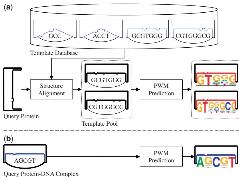
Figure 1. Prediction workflow incorporated in DBD2BS. (a) If the query is a DBD structure, DBD2BS searches the template database and uses structure alignment to generate appropriate DBD–DNA complex structures (the template pool) for PWM prediction. The DBD2BS reports both the potential DBDs on the query protein and the corresponding PWMs. The red binding interfaces indicate the potential DBDs. (b) If the query is a DBD–DNA complex, no extra action is required before PWM prediction. The DBD2BS reports the predicted PWMs, where the blue binding interface indicates that the DBD is known on the query rather than predicted.
