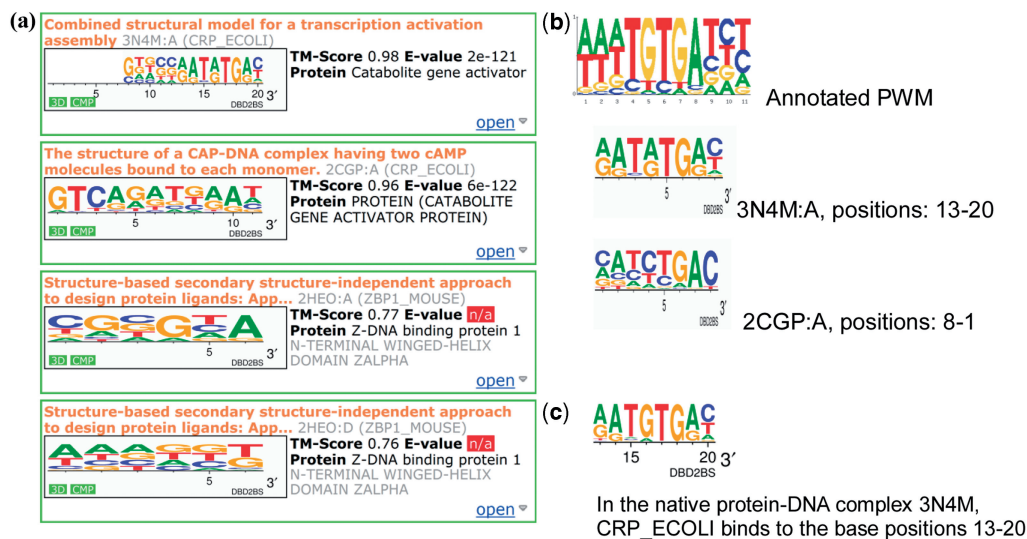
Figure 3. Case study using the catabolite gene activator of Escherichia coli .
