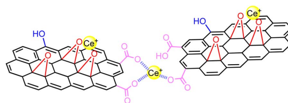
Scheme 1 Schematic representation of Ce^{+} grafting in the graphene oxide framework. For clarity, only a few functional groups are shown for clarity.
