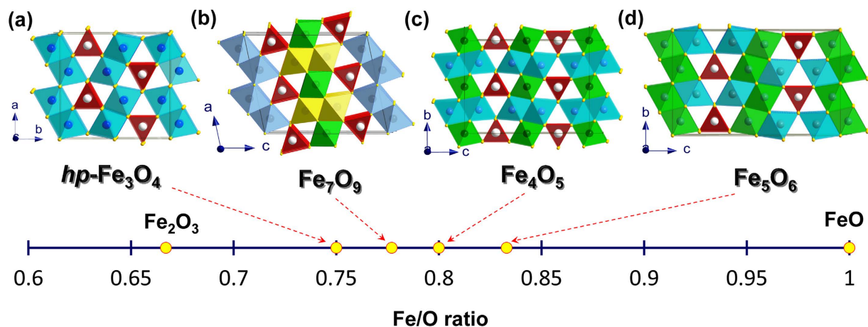
Figure 4. Comparison of unit cells of crystal structures of iron oxides. (a) High-pressure orthorhombic polymorph of \text{Fe}_3\text{O}_4 34 , (b) Monoclinic \text{Fe}_7\text{O}_9 polymorph discovered in the present work. (c) Orthorhombic Cmc polymorph of \text{Fe}_4\text{O}_5 discovered in ref. 13. (d) Orthorhombic Cmc polymorph of \text{Fe}_5\text{O}_6 discovered in ref. 14. Different colors of the octahedra denote different crystallographic sites for Fe ions.
