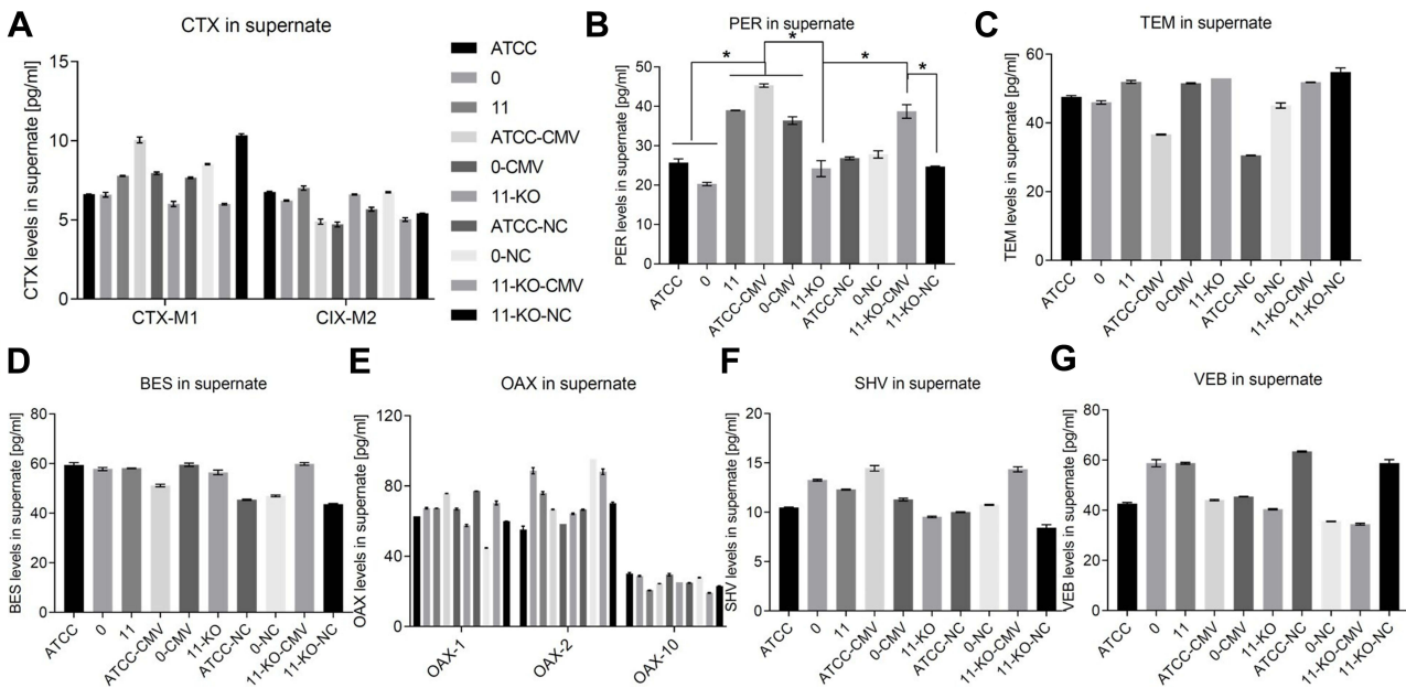
Figure 6 Determination of \beta -lactamase content in supernatant by ELISA.
