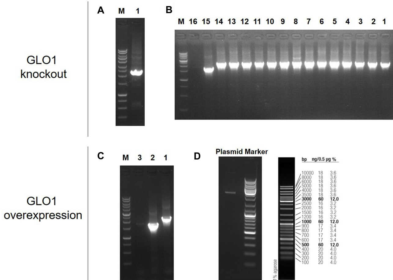
Figure 4 Verification of GloI gene knockout and overexpression in bacteria strain.
