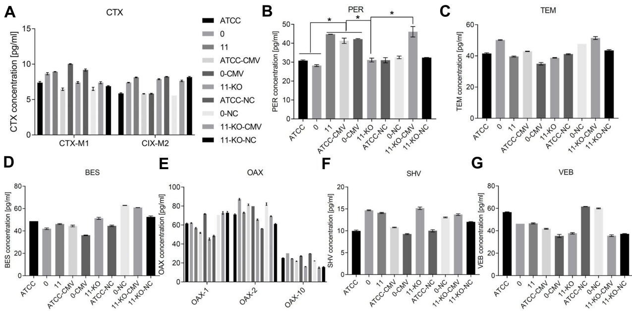
Figure 5 Determination of \beta -lactamase content in bacteria by ELISA.
