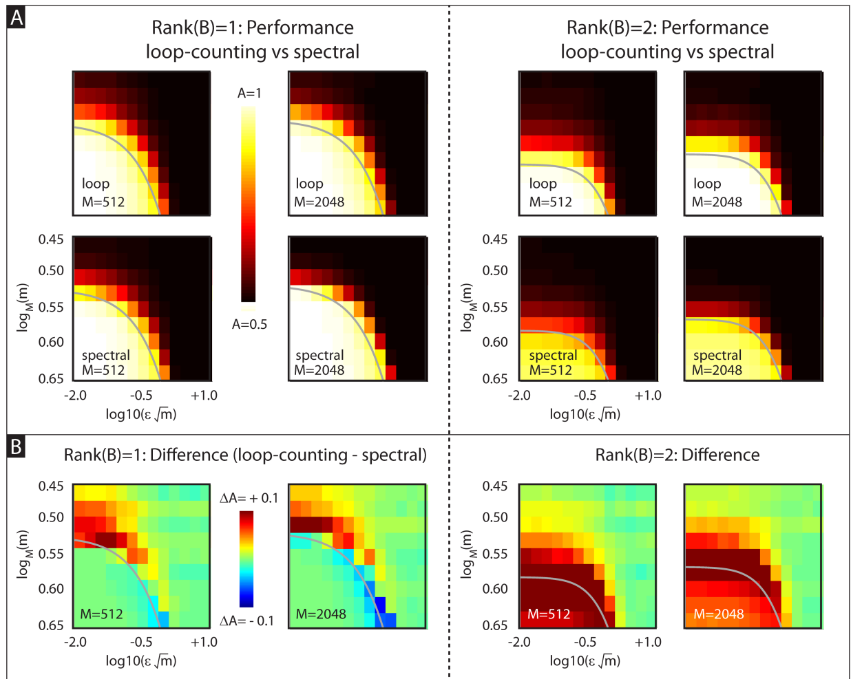
Fig 3. Performance of loop-scores vs spectral-biclustering applied to the planted-bicluster problem. For each instantiation of the planted-bicluster problem we choose an M , m , \epsilon and l ; we use these parameters to generate a random M \times M matrix D and embedded m \times m rank- l submatrix B with spectral noise \epsilon . For each instantiation, our algorithm produces a list of row- and column-indices of D in the order in which they are eliminated; those rows and columns retained the longest are expected to be members of B . To assess the success of our algorithm we calculate the auc A_R (i.e., area under the receiver operator characteristic curve) associated with the row-indices of B with respect to the output list from our algorithm. The value A_R is equal to the probability that: given a randomly chosen row from B as well as a randomly chosen row from outside of B , our algorithm eliminates the latter before the former (i.e., the latter is lower on our list than the former); We calculate the auc A_C for the columns similarly. Finally, we use A = (A_R + A_C)/2 as a metric of success; values of A near 1 mean that the rows and columns of B were filtered to the top by our algorithm, whereas values of A near 0.5 mean that our algorithm failed to detect B . In the top of Panel-A we show the trial-averaged auc A for our loop-counting method as a function of \epsilon\sqrt{m} and \log_M(m) . Results for l = 1 are shown on the left; l = 2 is shown on the right. Each subplot takes the form of a heatmap, with each pixel showing the value of A for a given value of \log_{10}(\epsilon\sqrt{m}) and \log_M(m) (averaged over at least 128 trials). The different subplots correspond to different values for M . Note that our loop-counting algorithm is generally successful when \log_{10}(\epsilon\sqrt{m}) \lesssim 0 and \log_M(m) \gtrsim 0.5 . In the bottom of Panel-A we show the analogous auc A for a simple implementation of the spectral method (see section A22 of S2 Text). In Panel-B we show the difference in trial-averaged A between these two methods (see colorbar for scale). Note that when l \geq 2 or the noise is small, our loop-score generally has a higher rate of success than the spectral method. On the other hand, there do exist parameters when l = 1 and \epsilon\sqrt{m} \sim 1 where the spectral method has a higher rate of success. In each panel the thin grey line shows the detection-boundary for our loop-counting method (calculated using m^3((2g_{l,\epsilon,m} - 1)) = \sqrt{2M^3} ).
