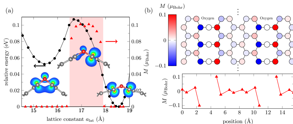
Figure 2. (a) Energy (black marks) and maximum magnetization (red marks) found in optimized GO nanoribbons of different widths, according to DFT calculations. The red shadowed area indicates non-zero magnetization for structures in the corresponding lattice constant range. The insets show partial charge densities around the oxygen atoms (red balls) and carbon atoms (gray balls) for three a_{\text{lat}} values: 15.5 Å, 17 Å, and 18.5 Å. (b) Magnetization at each atomic site in the unit cell of a GO layer of a_{\text{lat}} = 17 Å.
