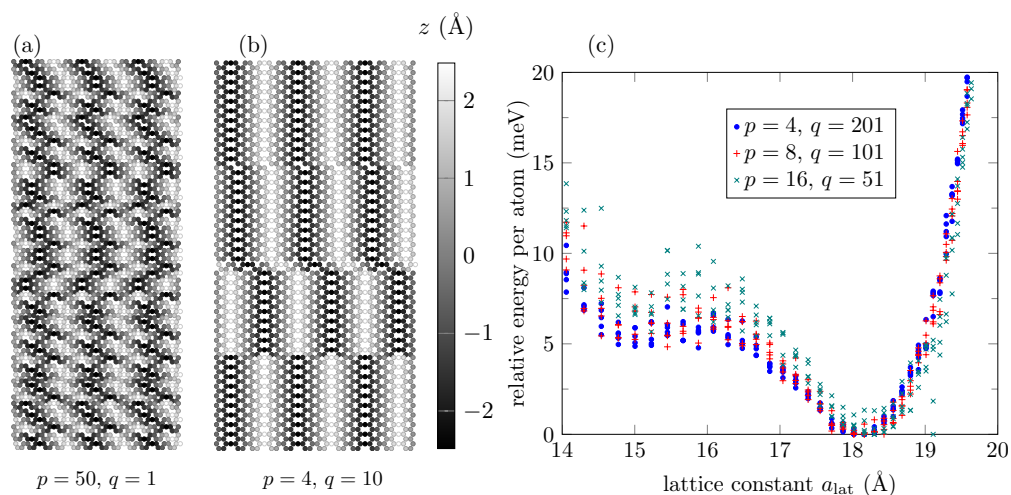
Figure 8. (a) Unit cell of a 50-AGNR with no ordered oxygen atoms over the surface ( q = 1 ). (b) Unit cell of a 40-AGNR with partially ordered oxygen atoms, with the order covering a length of q = 10 armchair lines. Periodicity is along the horizontal direction ( X -axis). Atoms are represented as balls in gray color levels to indicate their atomic height positions over the XY -plane. (c) Energy distribution of a 800-AGNR with partially ordered oxygen atoms at different levels, for q = 201 (highly ordered), 101, and 51.
