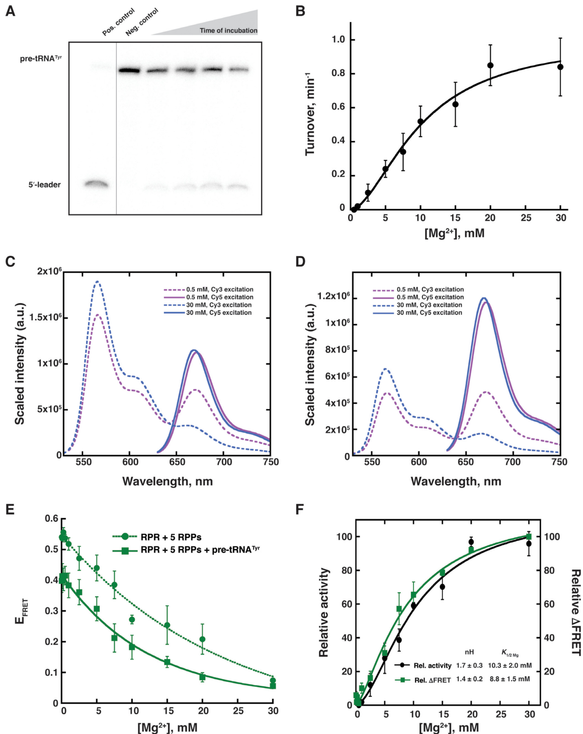
Figure 5. Effect of Mg 2+ on the activity and inter-domain interactions of Pfu RPR ext mP1 reconstituted with all 5 RPPs. (A) Representative data showing cleavage of \gamma - 32 P-ATP-labeled Escherichia coli ( Eco ) pre-tRNA Tyr by unlabeled Pfu RPR ext mP1 + 5 RPPs in 30 mM Mg 2+ and at 37°C during a 5-min time-course. For illustrative purposes, the gel was cropped to reposition non-adjacent lanes of interest; no other modifications were made to the image. (B) Mg 2+ -dependent increase in the activity of unlabeled Pfu RPR ext mP1. Average turnover numbers calculated from three independent initial velocity measurements are plotted against [Mg 2+ ], and the data were fit to the Hill equation. Dual-fluor-labeled Pfu RPR ext mP1 + 5 RPPs (C) without and (D) with Eco pre-tRNA Tyr shows a decrease in FRET from low (0.5 mM; purple) to high (30 mM; red) Mg 2+ . A representative spectrum from one trial at each Mg 2+ concentration is shown. Within each set, emission from direct Cy5 excitation was normalized against the sample with the highest signal. The same scaling factor was then applied to the corresponding emission spectrum obtained from Cy3 excitation (see Supplementary Figure S10 for additional data). (E) Mg 2+ -dependent increase in FRET efficiency for dual-fluor-labeled Pfu RPR ext mP1 + 5 RPPs without (dotted line) and with (solid line) Eco pre-tRNA Tyr . Average FRET efficiency from three independent measurements is plotted against [Mg 2+ ]. (F) Comparison of relative turnover numbers (black) and \Delta FRET values (green solid line). Data for Pfu RPR ext mP1 + 5 RPPs + Eco pre-tRNA Tyr were fit to the Hill equation to obtain the n_H (Hill coefficient) and K_{1/2, Mg} values in the inset (see Supplementary Figure S11 for additional data).
