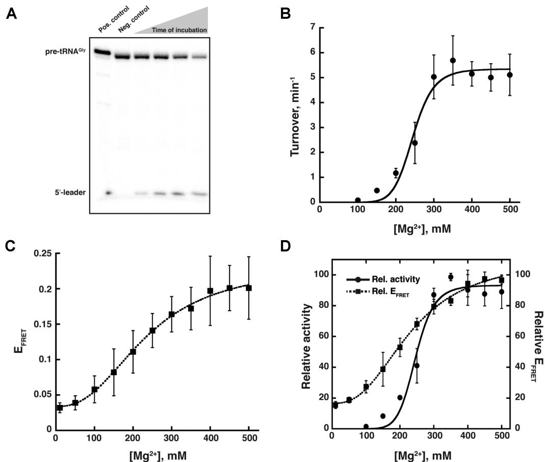
Figure 4. Effect of Mg 2+ on the activity and inter-domain interactions of Pfu RPR ext mP1. (A) Representative data showing cleavage of \gamma - 32 P-ATP-labeled Thermus thermophilus ( Tth ) pre-tRNA Gly by unlabeled Pfu RPR ext mP1 in 450 mM Mg 2+ and at 37°C during a 20-min time-course (also, see Supplementary Figure S4 and S5). (B) Mg 2+ -dependent increase in the activity of unlabeled Pfu RPR ext mP1. Average turnover numbers calculated from four independent initial velocity measurements are plotted against [Mg 2+ ]. (C) Mg 2+ -dependent increase in FRET efficiency for dual-fluor-labeled Pfu RPR ext mP1. Average FRET efficiencies obtained from three independent measurements are plotted against [Mg 2+ ] (see Supplementary Figure S6 for additional data). (D) Overlay of turnover number (solid line) and FRET efficiency (dashed line), which shows that FRET efficiency correlates with the rate of catalysis as a function of [Mg 2+ ]. Relative activity and E FRET values were obtained by normalization against the highest turnover number or FRET efficiency, respectively; since this reference value was not always at the same concentration of Mg 2+ among the replicates, there is minor variability between panels B or C versus D but the trends are highly similar. In instances where error bars are not seen, the errors are smaller than the symbols used.
