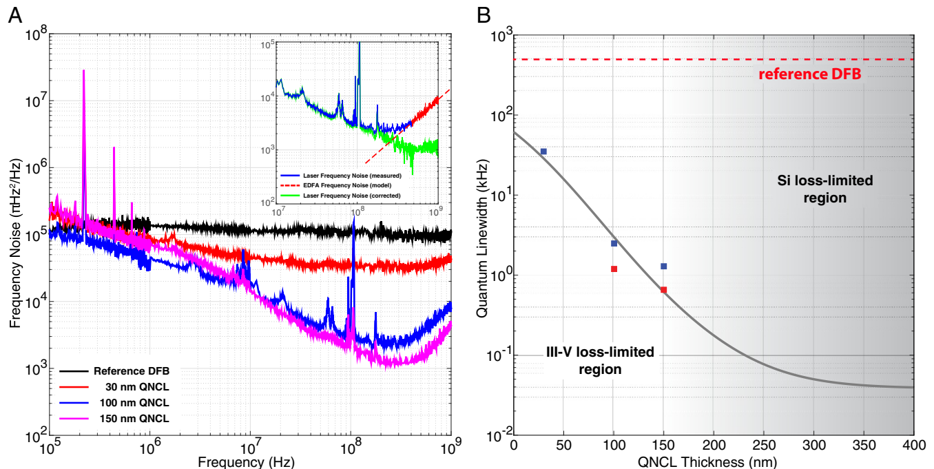
Fig. 4. Experimental results. (A) Measured PSD (in units of equivalent white noise linewidth, \pi\text{Hz}^2/\text{Hz} ) of the frequency noise of Si/III-V lasers with three different values of QNCL thickness (30, 100, and 150 nm). Plotted alongside for comparison is the frequency noise spectrum of a commercial DFB (black trace), also used for measurement calibration. All the traces of the Si/III-V lasers were taken at the same current increment ( \sim 30 mA) from their respective threshold, while that of the reference DFB was at its maximum operating current. (A, Inset) Numerical correction for the EDFA noise for the case of the 100 nm QNCL. The measured noise above \sim 300 MHz is fitted to S_{\Delta\nu}(f) = af^b + S_0 (red dashed line), with a , b being fitting coefficients and S_0 a frequency-independent term (i.e., white noise). Subtracting the frequency-dependent term (i.e., af^b ) from the measured noise yields the corrected spectrum (green line). (B) Experimental quantum linewidths (blue markers) plotted against the theoretical trend line (gray trace), as calculated via Eq. 9 for Q_{\text{Si}}=10^6 . To set the vertical axis, the linewidth of the reference DFB (red dashed line), measured at an equivalent pump rate, is used to convert from relative (Fig. 3B) to absolute linewidth. Red markers represent linewidth estimates for the cases of the numerically filtered EDFA noise. The gray-shaded area corresponds to the theoretically estimated Si loss-limited region.
