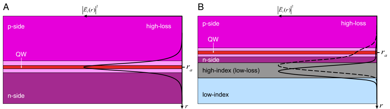
Fig. 1. Concept illustration of the modal control of spontaneous emission in a semiconductor laser. (A) Cross-sectional structure of a generic, electrically pumped semiconductor laser along with a simulated example of the transverse distribution of the electric field intensity, |\bar{E}_e(\bar{r})|^2 , of the laser mode. (B) In a departure from the standard semiconductor laser design, the laser mode is “pulled” into and is guided by a transversely proximal to the active region layer. The low-loss nature of the latter is key for offsetting the resulting decrease in modal gain. The location of the active region in the evanescent tail of the mode enables leveraged (i.e., exponential) control over |\bar{E}_e(\bar{r})|^2 and, thereby, of the spontaneous emission rate into the laser mode, as showcased by two simulated examples (solid and dashed black lines).
