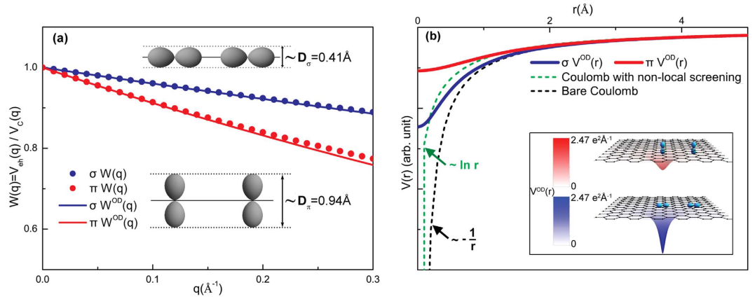
Figure 1. (a) Orbital-dependent Coulomb matrix elements for \pi and \sigma orbitals. The points indicate the calculated W(q) from Eq. (6), and the solid lines are the orbital-dependent W^{OD}(q) from Eq. (7). (b) A collection of four types of potentials to describe electron-hole interaction. The form of Coulomb interaction with non-local screening is given in ref. 35 by Keldysh, and ref. 36 by Cudazzo, Tokatly and Rubio. The orbital dependent e-h interactions in both \pi and \sigma states are shown in inset of Fig. 1b.
