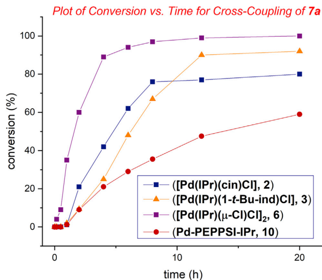
Figure 2. Kinetic Profile of Suzuki-Miyaura Cross-Coupling of Amides
