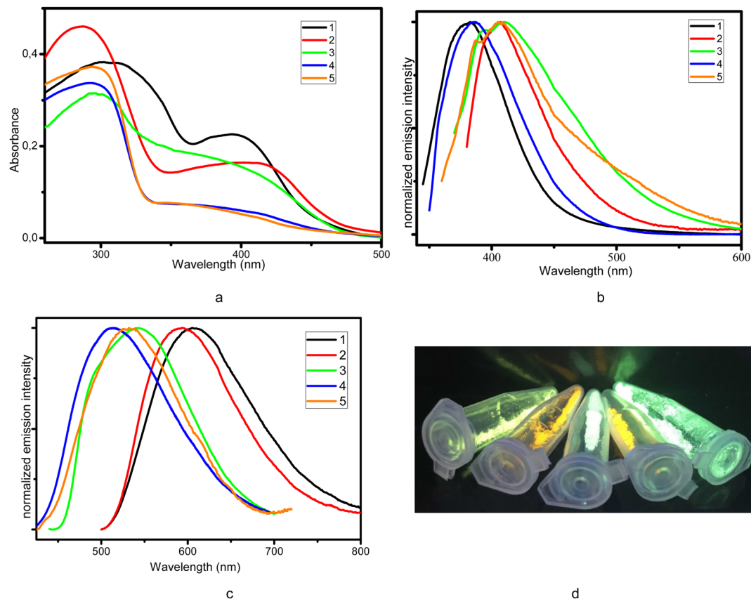
Fig. 2 Absorption spectra of solid state complexes (a), normalized emission spectra of THF solution ( 10^{-5} M) (b) and solid polycrystalline samples (c) of 1–5 at room temperature (above) and luminescence images of 1–5 under UV lamp (d).
