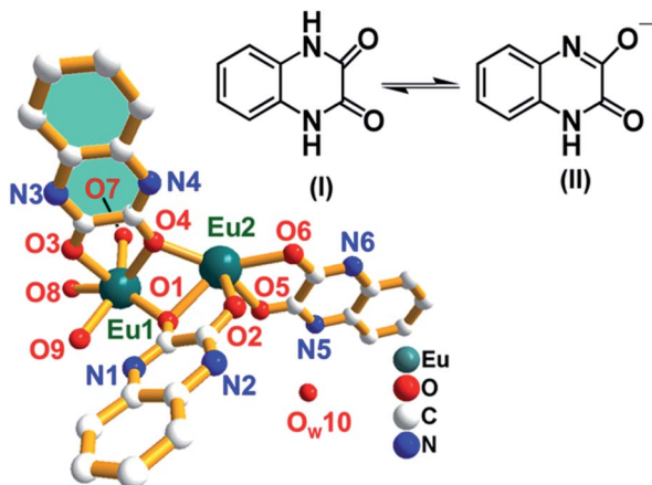
Fig. 2 The asymmetry unit of complex 1 [\text{Eu}_2\text{O}_2(\text{OH})(\text{HQXD})(\text{H}_2\text{-QXD})_2]\cdot\text{H}_2\text{O} with isomeric forms of the ligand. The H atoms are omitted for clarity. Color code: green-blue, Eu; blue, N; red, O; white, C.
