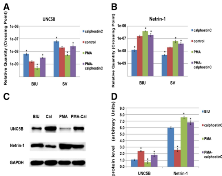
Figure 6 Expressions by RT-PCR and western blot in bladder cells with drugs. (A) & (B) Quantitative real-time PCR (RT-PCR) were used to evaluate netrin-1 & UNC5B's expression in treatment of cells (BIU & SV) with drugs- PMA (PKC \alpha agonist) and calphostin C (PKC \alpha inhibitor). The results showed that the cells were significantly inhibited by calphostin C (24 h) in netrin-1's expression and promoted by PMA (24 h), and cells were first promoted, and then inhibited by PMA (4 h) then calphostin C (24 h). While UNC5B was opposite. (C) Confirmation of netrin-1 down-regulation with calphostin C and up-regulation with PMA by western blot. (D) The relative protein expression of netrin-1 & UNC5B in treatment of cells with drugs, GAPDH as an internal control ( P < 0.05 ). *P < 0.05 compared with BC cell line BIU (paired t -test).
