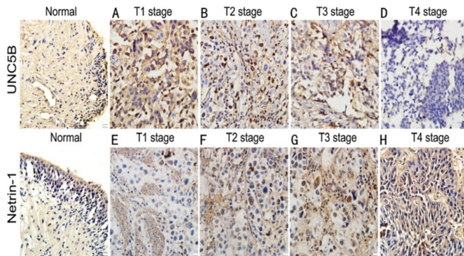
Figure 3 Representative images from immunohistochemical staining in different histological stages UNC5B was localized at cytoplasm and netrin-1 was mainly in cell nucleus and partly in cell cytoplasm of tumor tissues with granular brown staining. Almost all T1 tumor tissues showed strong UNC5B staining intensity. UNC5B expression in stage T4 was significantly less than in stage T1–T3 specimens (Figure 3A, B, C & D) ( P = 0.021 ). While netrin-1 showed strong expression in stage T4 than other stages (T3, T2 & T1) and was associated significantly with pT stage (Figure 3E, F, G & H) ( P = 0.013 ). Representative tissue sections with different immunointensity of UNC5B protein in A T1, B T2, C T3 & D T4. E Low level of netrin-1 expression in T1, H High level of netrin-1 expression in T4, F & G represent T2 & T3. Magnification \times 400 . * P < 0.05 compared with stage normal bladder tissues (paired t -test).
