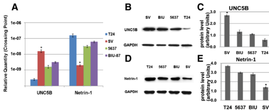
Figure 5 Expressions by RT-PCR and western blot in bladder cell lines. (A) Netrin-1 & UNC5B mRNA expression in four bladder cell lines (T24, SV, 5637, and BIU-87) was assayed using quantitative real-time PCR. To normalize Netrin-1 & UNC5B expression, \beta -actin was used as internal control. Each expression level was shown as mean + SD. UNC5B expression was significantly greater in SV cells than in 5637, T24 or BIU-87, while netrin-1 was lower in SV than in BC cell lines. *P < 0.05 compared with BC cell lines including 5637, T24 and BIU-87 (paired t -test). (B) UNC5B & (D) Netrin-1 expression at protein level in different cell lines (SV, BIU, 5637 and T24) were analyzed by western blots with 50 \mu g protein extracts. GAPDH was selected to be endogenous control. The differences in UNC5B expression between 5637, T24 and BIU-87 were significant. SV cells represent bladder normal cell lines of which UNC5B expression is the most, the others are BC cell lines, and netrin-1 expresses the least in SV. (C) & (E) The ratio between the optical density of UNC5B & netrin-1 and GAPDH of the same tissue was calculated and expressed graphically ( P < 0.05 ). *P < 0.05 compared with BC cell lines (paired t -test).
