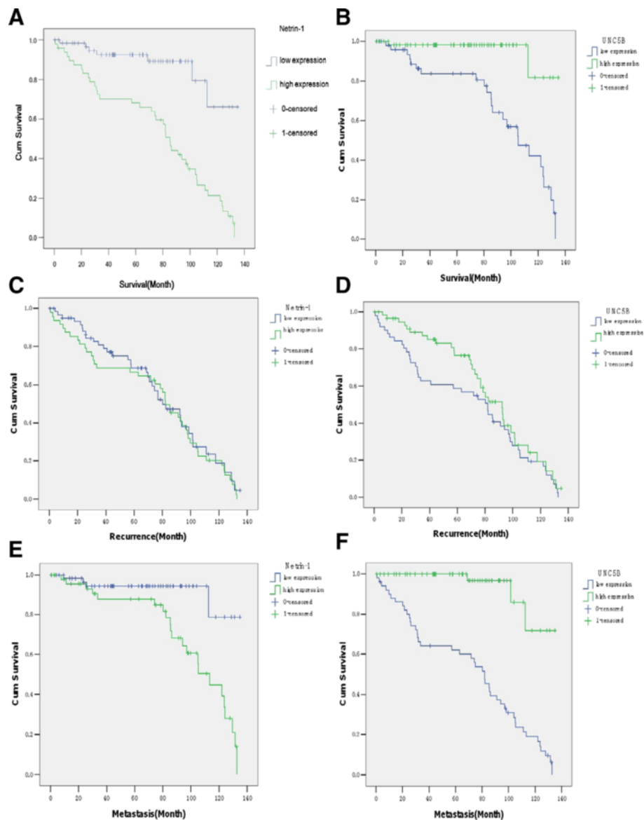
Figure 4 Survival, recurrence and metastasis curve analysis by the Kaplan-Meier method. (A) Patients with intense netrin-1 expression had significantly shorter median survival time (76.624 months) than those with weak netrin-1 expression (117.981 months) through log-rank univariate analysis ( n = 120 , P < 0.01 ). (B) Patients with weak UNC5B expression had significantly shorter median survival time (96.881 months) than those with intense UNC5B expression (128.939 months) ( P < 0.01 ). (C) Recurrence curve analysis indicated that the difference was not statistically significant with intense netrin-1 expression (74.463 months) and lower expression (79.505 months). ( P > 0.01 ) (D) The difference was not statistically significant in more (84.47 months) and less (69.225 months) UNC5B expression by recurrence curve analysis. ( P > 0.01 ) (E) Patients with intense netrin-1 expression had significantly shorter median metastasis time (100.836 months) than those with weak netrin-1 expression (124.946 months). ( P < 0.01 ) (F) Patients with weak UNC5B expression had significantly shorter median metastasis time (71.243 months) than those with intense UNC5B expression (125.957 months). ( P < 0.01 )
