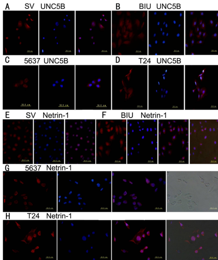
Figure 7 Detection of UNC5B expression by immunofluorescence in four cell lines (SV, BIU, 5637 & T24) (A & E) SV, (B & F) BIU, (C & G) 5637, (D & H) T24. (A, B, C & D) The expression of UNC5B located in cytoplasm (red color). The blue ones were cell nucleolus. Other ones are transmission light figures. From these figures we can see cells' form clearly. UNC5B location was almost the same in SV, 5637, T24 & BIU-87 bladder cancer cells lines. (E, F, G & H) The localization in four cell lines (SV, BIU, 5637 & T24) of netrin-1 was found by immunofluorescence mainly in cell nucleus and partly in cell cytoplasm.
