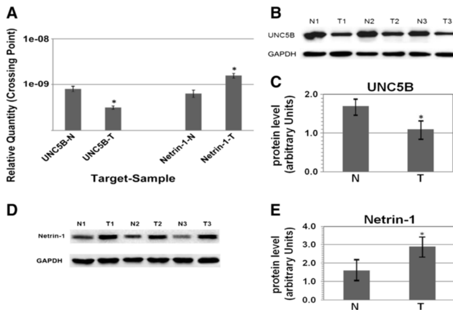
Figure 1 Expression by RT-PCR and western blot in BC tissues (T) and normal bladder tissues (N). (A) The average netrin-1 & UNC5B expression \pm SD for all studied tumors (120 cases) and their corresponding normal tissues (40 cases) by RT-PCR, bar graphs describe significant UNC5B down-regulation and netrin-1 up-regulation in T in comparison with N ( P < 0.05 ), \beta -actin as an internal control. (B) UNC5B protein was detected by western blot in 40 pair tissues and band intensities indicate UNC5B expression conspicuously lower in T comparing with N. GAPDH was used as a loading control. (C) The ratio between the optical densities of UNC5B & GAPDH in the same tissue was calculated and expressed graphically. Significant differences of UNC5B expression between T & N were analyzed statistically and UNC5B expression was obviously greater in N ( P < 0.05 ). (D) Netrin-1 protein was detected by western blot and increased in T. (E) The relative protein expression of netrin-1, GAPDH as an internal control ( P < 0.05 ).
