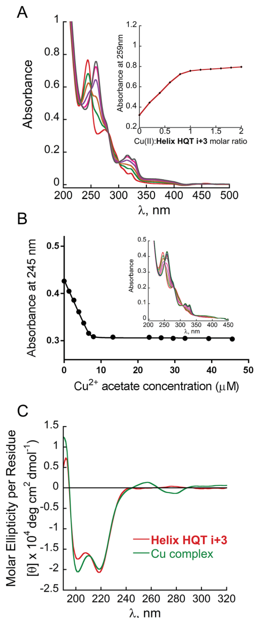
Fig. 1 (A) UV-Vis spectra and peptoid-to-metal ratio plot for the titration of Helix HQT i + 3 with \text{Cu}^{2+} . The peptoid (17 \mu\text{M} ) in MeOH : H 2 O 4 : 1 solution was titrated with 2 \mu\text{L} aliquots of a metal ion (5 mM in H 2 O) in multiple steps (red = free ligand, black = metal complex). (B) Non-linear regression fit and UV-Vis spectra for the titration of Helix HQT i + 3 with \text{Cu}^{2+} . The peptoid (7 \mu\text{M} ) in MeOH : H 2 O 1 : 5 solution was titrated with 2 \mu\text{L} aliquots of a metal ion (2 mM in H 2 O) in multiple steps (red = free ligand, black = metal complex). (C) CD spectra of Helix HQT i + 3 (100 \mu\text{M} in MeOH : H 2 O 4 : 1) before (red) and after (green) the addition of 1 equivalent \text{Cu}^{2+} .
