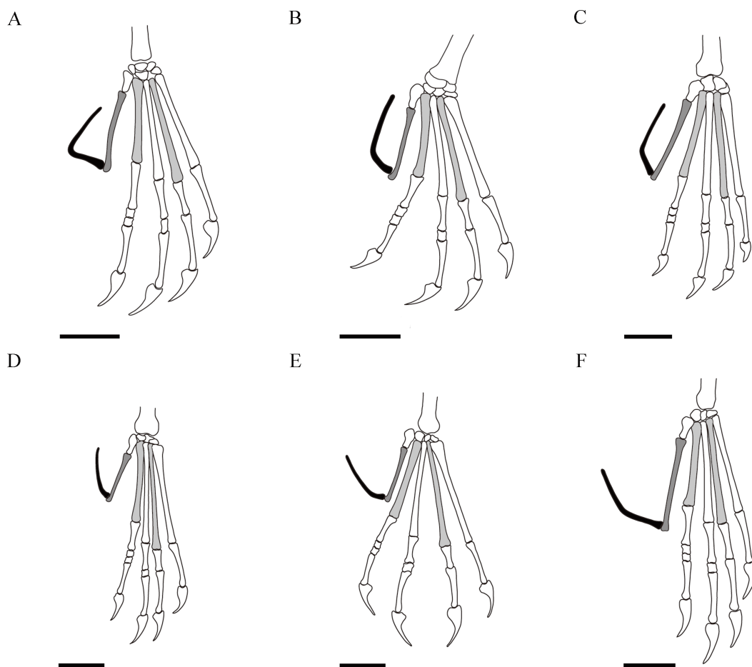
Figure 6 Reconstructions of wukongopterid feet with all metatarsals II of the same size. Showing metatarsals II and IV in light grey, first phalanges of pedal digit V in dark grey and second phalanges in black. Scale bars: 10 mm. (A) Wukongopterus (based on Wang et al., 2009). (B) Darwinopterus linglongtaensis (based on Wang et al., 2010). (C) Darwinopterus robustodens (based on Lü et al., 2011a). (D) Holotype of Kunpengopterus sinensis (based on Wang et al., 2010). (E) Kunpengopterus sinensis (IVPP V 23674). (F) IVPP V 18403/ZMNH M8802 (wukongopterid with eggs, based on Lü et al., 2011b; Wang et al., 2015).
