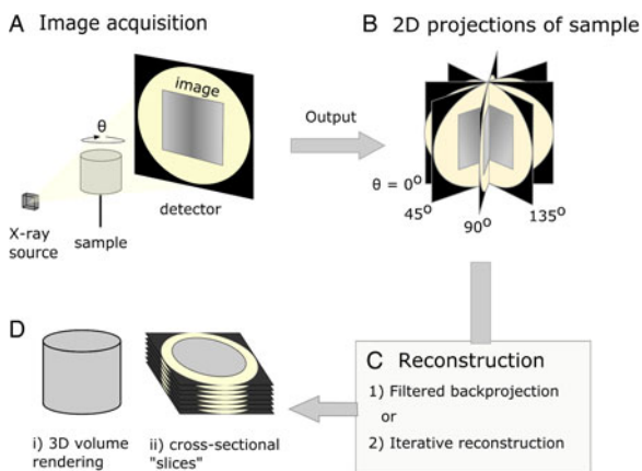
Fig. 1. Diagrammatic representation of X-ray micro-computed tomography workflow. (A) Basic illustration of tomographic apparatus, including the X-ray source, detector and sample. Projection images are made as the sample is rotated at increments through \theta . (B) The raw output of the tomogram is a series of projections of the sample taken at different angles. (C) Projections are digitally ‘reconstructed’; two commonly used approaches are filtered backprojection and iterative reconstruction. Reconstruction algorithms output a dataset which is suitable for analysis. (D) The sample may be viewed in a virtual environment in a variety of ways, including as a 3D rendered volume (Di). Alternatively, 2D cross-sections, or ‘slices’ (Dii), of the sample may be viewed.
