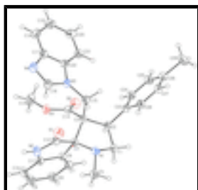
Fig. 1. The molecular structure of the title compound, showing the atom-numbering scheme. Displacement ellipsoids are drawn at the 30% probability level
