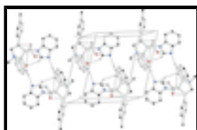
Fig. 2. Molecular packing of the title compound, viewed down the a axis; H-bonds are shown as dashed lines. For the sake of clarity, H atoms, not involved in hydrogen bonds, have been omitted
