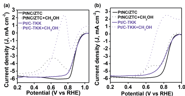
Fig. 5 ORR polarization curves of PtNC/ZTC and Pt/C-TKK in the absence (solid line) and presence (dotted line) of 0.1 M \text{CH}_3\text{OH} at a rotation rate of 1600 rpm in (a) alkaline and (b) acid media.
