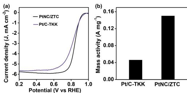
Fig. 4 (a) RDE ORR polarization curves at 1600 rpm and (b) mass activity at 0.8 V of PtNC/ZTC and Pt/C-TKK in 0.1 M \text{HClO}_4 .
