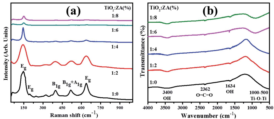
Fig. 5 (a) Raman spectra and (b) FTIR profiles of TiO 2 and co-doped TiO 2 products.
