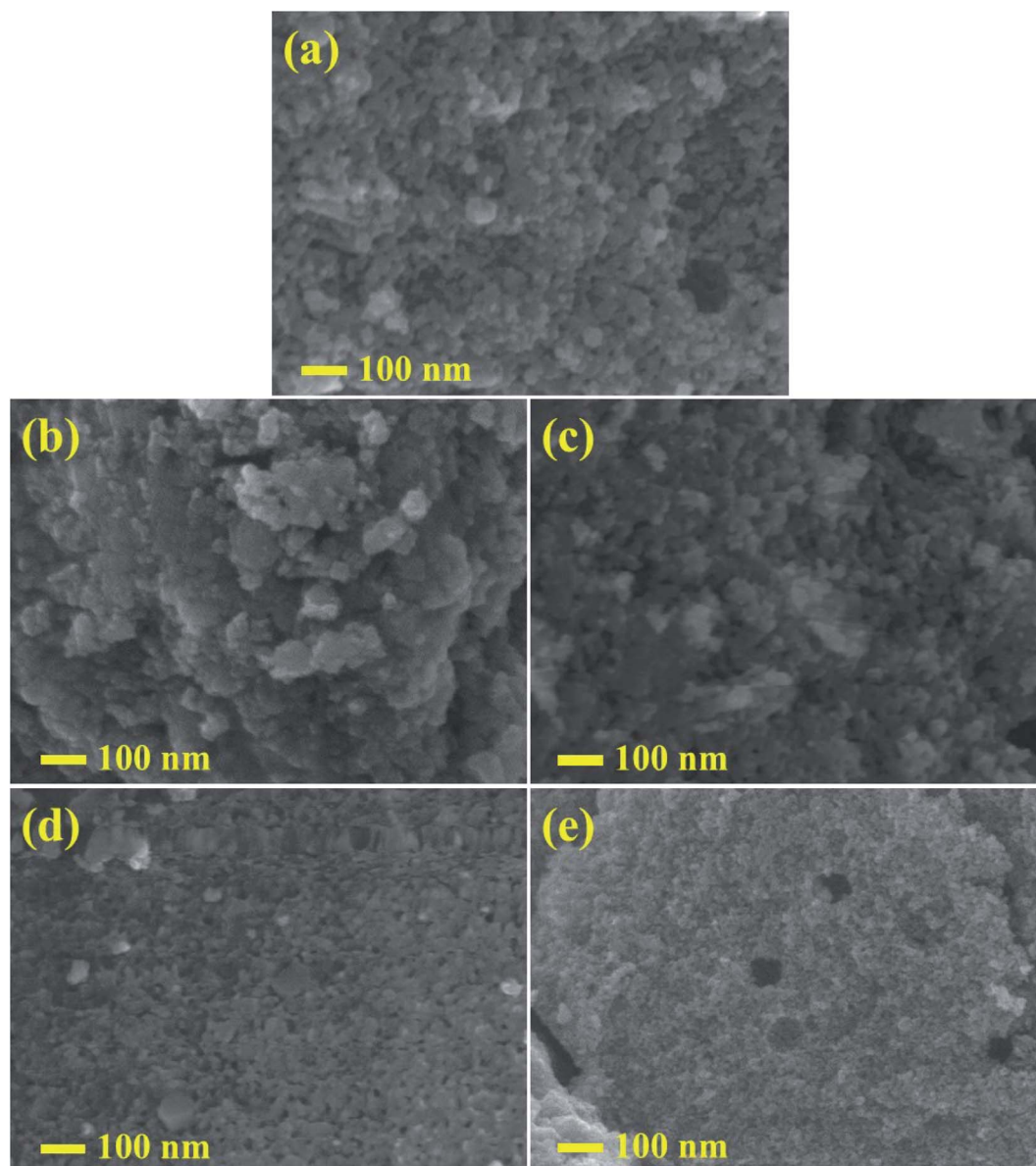
Fig. 6 (a–e) FESEM images of pure and ZA (2, 4, 6 and 8 wt%) doped TiO 2 nanostructures, respectively.
