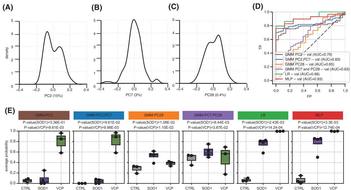
FIGURE 2 Machine-learning based methods enable automated discrimination of VCP- and SOD1-mutant groups from control groups.
