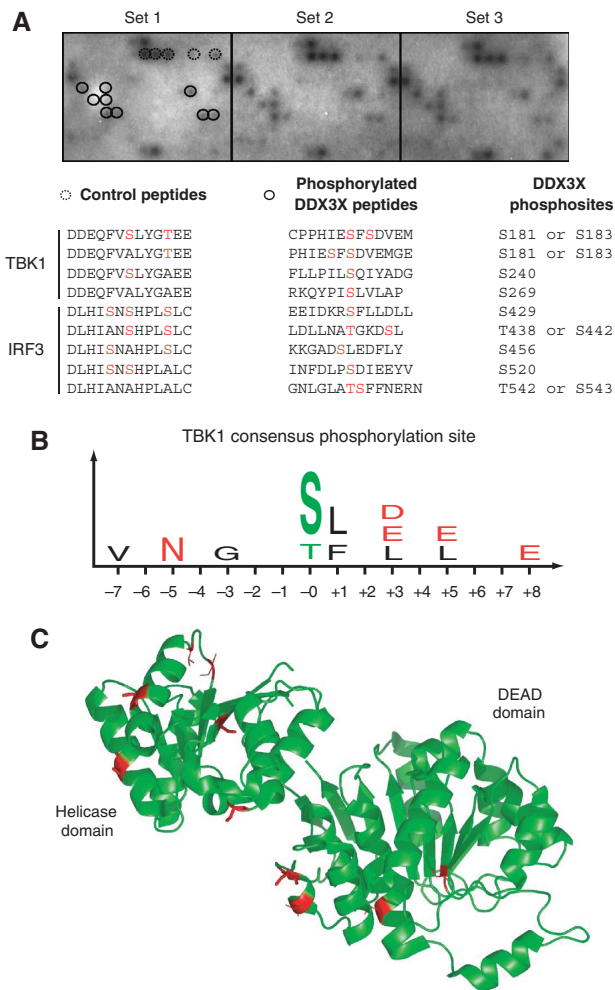
Figure 7 Mapping of the TBK1 phosphorylation site in DDX3X. (A) Peptides derived from DDX3X or control peptides derived from TBK1 or IRF3 along with alanine mutants were incubated with TBK1 in the presence of [ \gamma - ^{32} P]ATP. Each array contained a total of 82 peptides spotted in triplicate. (B) Phosphorylation sites obtained from the peptide array (see also text) were used to build a TBK1 phosphorylation consensus sequence. (C) Putative DDX3X phosphorylation sites were mapped onto the structure of a truncated version of DDX3X.
