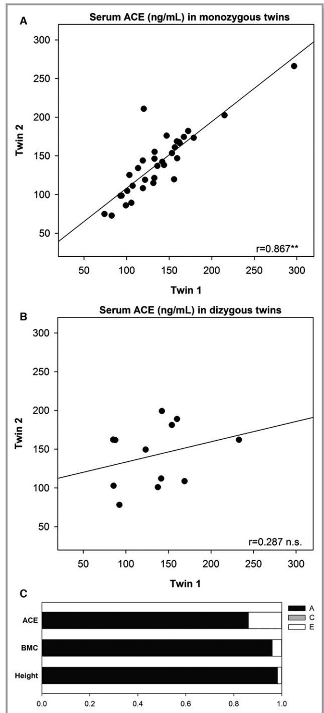
Figure 5. Intrapair correlation of ACE serum concentrations in monozygotic (A) and dizygotic (B) twins (** P < 0.01 ). Estimated heritability (C) for ACE serum concentrations in comparison with estimates for bone mineral content (BMC) and height: “A” additive genetic effects, “C” common environmental influences, and “E” unique environmental influences. ACE indicates angiotensin-converting enzyme.
