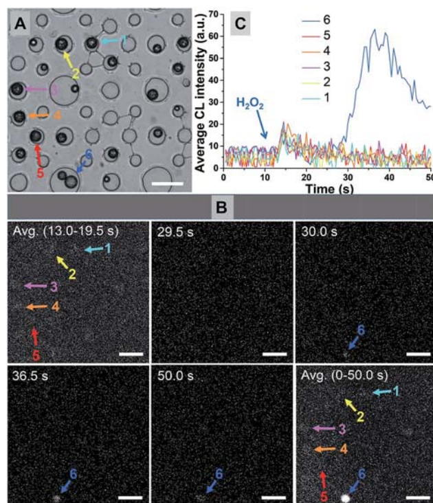
Fig. 2 (A) Bright field image (scale bar: 100 \mu m) of multiple microbeads trapped in the microwells. (B) Snapshots at different moments and the averaged CL images upon reaction with H_2O_2 (scale bar: 100 \mu m). (C) Representative CL kinetics curves of six microbeads showing weak (1–5) and strong (6) emission, respectively.
