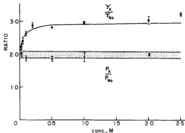
FIGURE 6. Concentration dependence of channel selectivity. The channel selectivity was studied as a function of salt concentration with two different types of measurements. The channel conductance for K^+ or Na^+ under symmetrical conditions was measured as in Fig. 4, and the ratios were calculated at the same concentrations (filled circles). Alternatively, the permeability ratio was measured under bi-ionic conditions as in Fig. 5 (open circles). Each permeability ratio represents the mean \pm SEM of three determinations, each on a different membrane. The continuous upper curve is drawn as in Fig. 4, with the ratio of K^+ and Na^+ conductances and with correction for activity coefficient differences at equal concentrations of NaCl and KCl. The stippled region represents the range of permeability ratio predicted by a single-ion model, given the errors of the parameters describing the conductance-activity relation (Table II).
