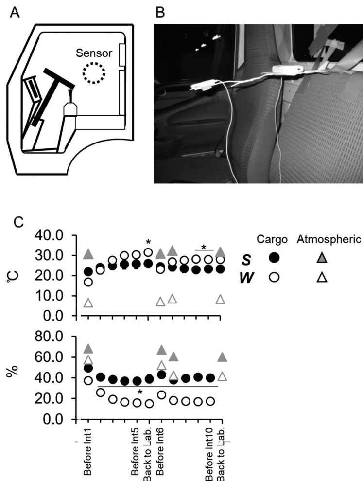
Fig. 3. Measurement for environmental conditions in the cockpit in summer ( S ) and winter ( W ). A place to measure it by a thermistor and a hygrometer are represented as an illustration (A) and a picture (B). C: Temperature (upper) and relative humidity (lower panel) in the cockpit and atmospheric air, which were adapted as the data in Wakayama city announced from Japan Meteorological Agency, are shown as a figure. Values are means (SE) for 6 subjects. *Significant differences between S and W at the level of p < 0.05 .
