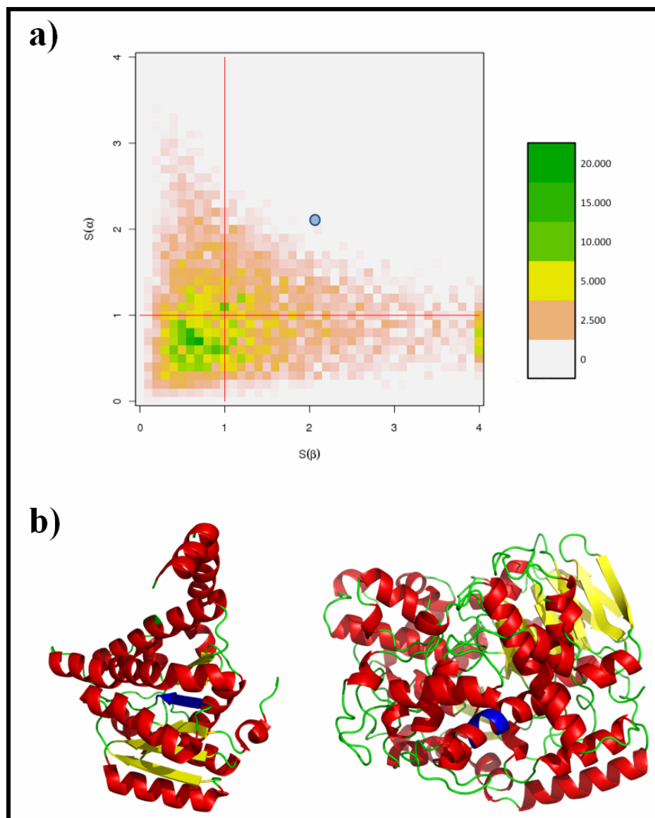
Figure 1: (a) Distribution of adequacy scores S(\alpha) and S(\beta) of chameleon sequence fragment of length 4. The legend gives the occurrence number of observed fragments. (b) example of the chameleon sequence fragments MLIL found (left) in a \beta -strand of Guinea pig 11 beta-hydroxysteroid 2 dehydrogenase type 1 (PDB code 1XSE) and in an \alpha -helix of a hyperthermophilic tungstoperin enzyme 2 aldehyde ferredoxin oxidoreductase (PDB code 1aor). The blue point in (a) represents the scores of example (b).
