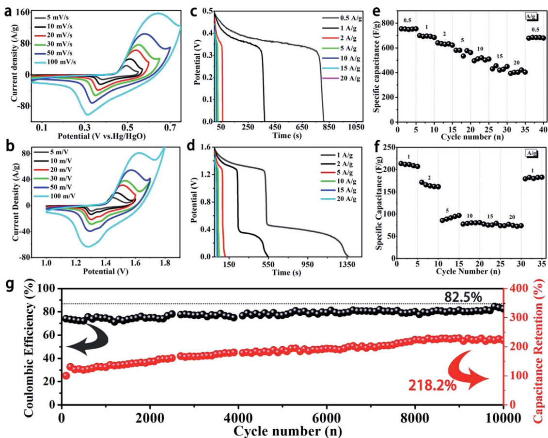
Fig. 3 Electrochemical performances of the sample \alpha\text{-Ni}(\text{OH})_2 in a three-electrode system and two-electrode system. (a and b) CV curves, (c and d) galvanostatic discharge–charge curves, (e and f) rate performance and (g) cycle testing of \alpha\text{-Ni}(\text{OH})_2/\text{NF}/\text{AC} device at 5 \text{ A g}^{-1} .
