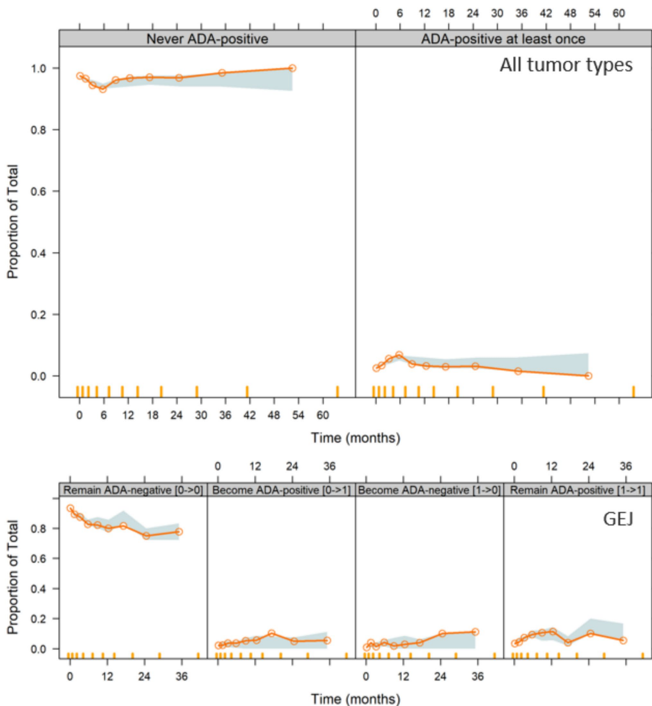
Fig. 5 Visual predictive check for the population discrete-time Markov model. Top panel: all tumor types. Bottom panel: GC/GEJC tumors (in JAVELIN Gastric 100). The open circles show the
