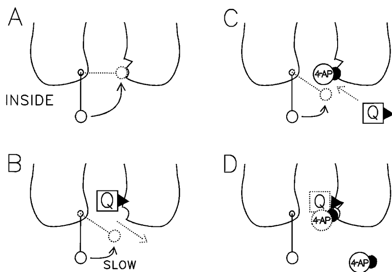
FIGURE 11. A schematic diagram of the physical interactions between quinidine, 4-AP, and hKv1.5. (A) Normal channel closing is shown by the activation gate swinging from open ( solid ) to shut ( dotted ). (B) Open channel block by quinidine results in a quinidine-blocked state, impeding the activation lid from closing the channel and slowing channel deactivation. (C) 4-AP has access to open channels and can keep the channels in a nonconducting 4-AP-blocked state when 4-AP is trapped within the channel. 4-AP-trapped channels prevent complete closing of the activation lid ( dotted ) and allow quinidine access to its binding site, which is close to that of 4-AP. (D) 4-AP and quinidine can coexist at binding sites within the inner mouth of the channel. Allosteric modulation of quinidine binding by the presence of 4-AP, and vice-versa, occurs. This reduces the apparent K_d for quinidine \sim 20 -fold and allows reopening of silent channels in the presence of high concentrations of 4-AP.
