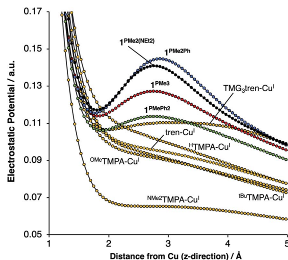
Fig. 7 One-dimensional electrostatic potential map along the canonical z-axes of the \text{Cu}^{\text{I}} complexes.
