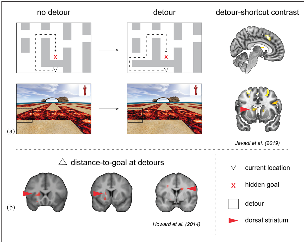
Figure 1. Dorsal striatum activity is correlated with the change in distance to goal at detours.
