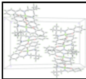
Fig. 2. Crystal packing of (I), viewed along the a axis showing the stacking of the molecules along the b direction. The disordered ethanol molecule is omitted for clarity.
