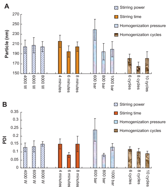
Figure 1 Optimization for the technical preparation of the β-E-NLCs. Stirring power, stirring time, homogenization pressure, and homogenization cycle are used as the factors, and the particle size (A) and PDI (B) are used as the index.
